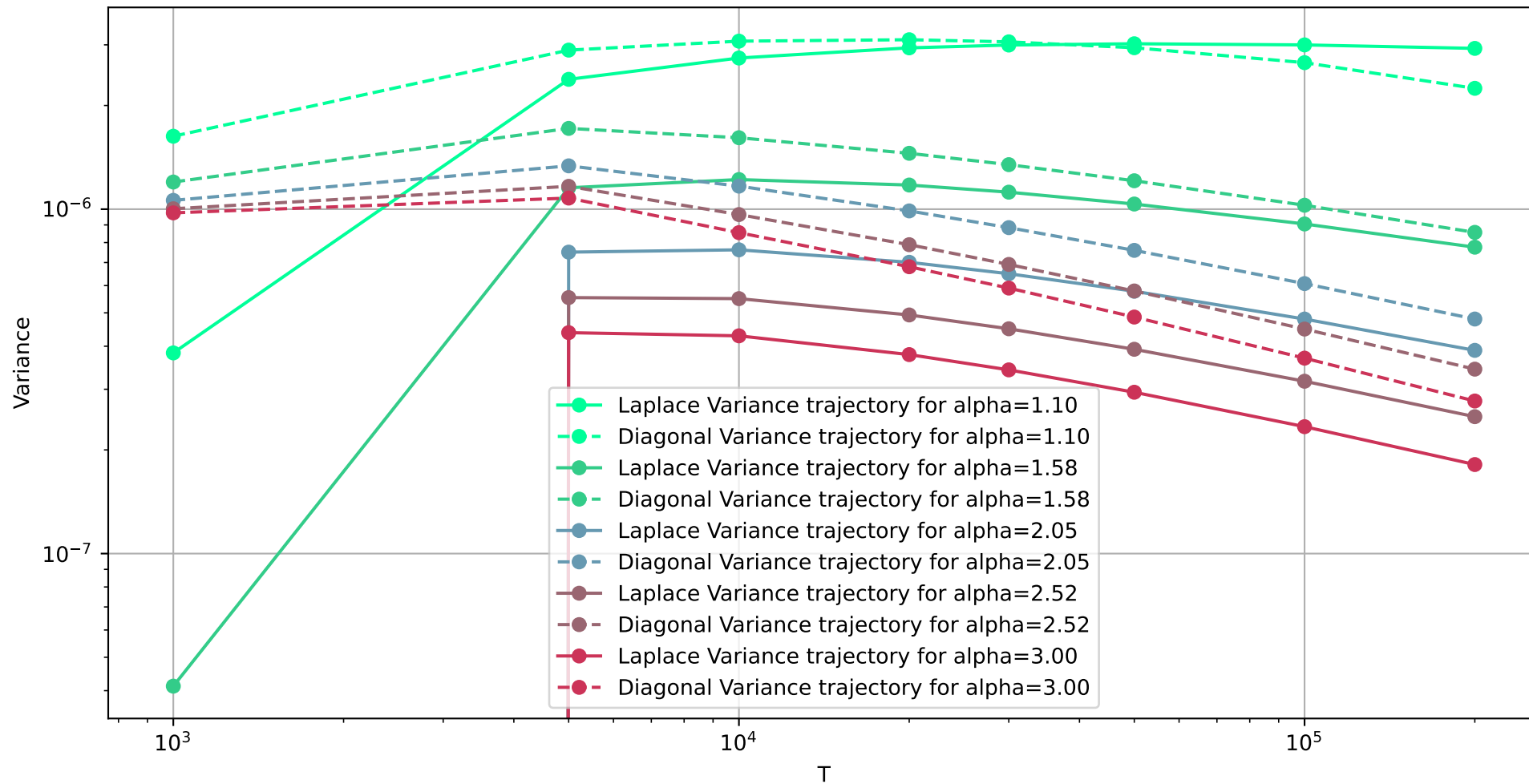
Variance Trajectories for Different Alphas
