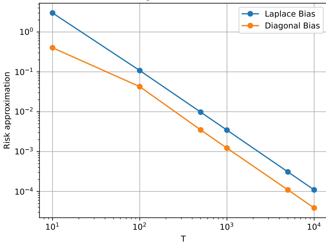
Components of Laplace approximation vs Diagonal approximation for linear s sigma=0.5, beta=2
