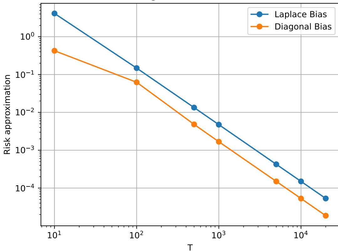
Components of Laplace approximation vs Diagonal approximation for linear sc sigma=0.5, beta=2
