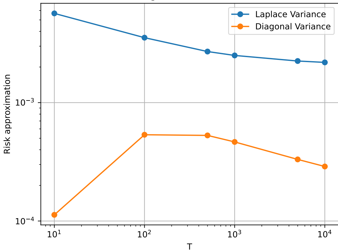
Components of Laplace approximation vs Diagonal approximation for linear sigma=0.5, beta=2
