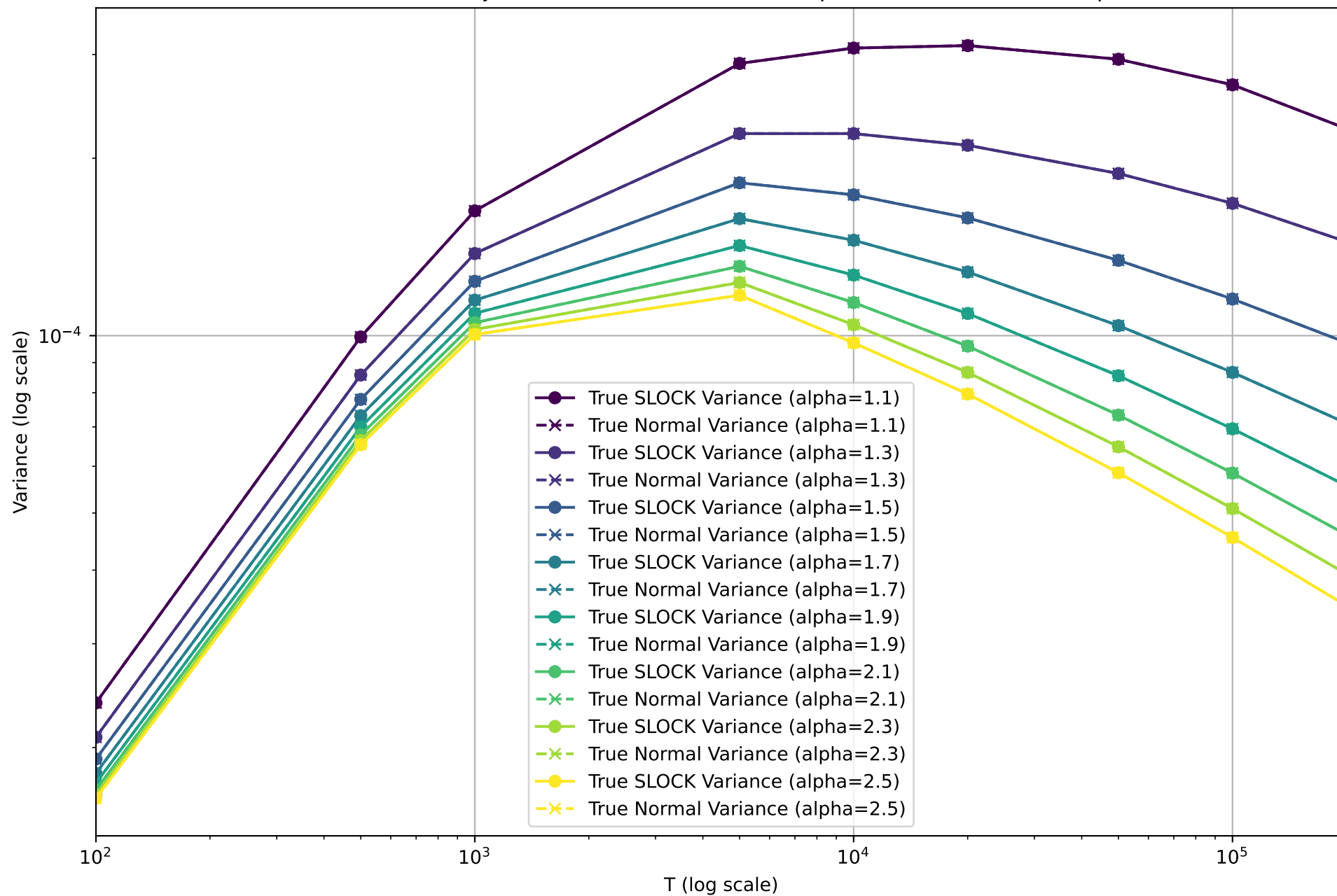
True Variance Trajectories (SLOCK vs Normal) optimized eta, different alphas
