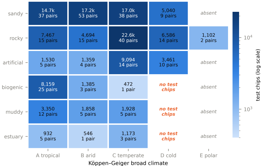
GCL_FCS30 coastline type
