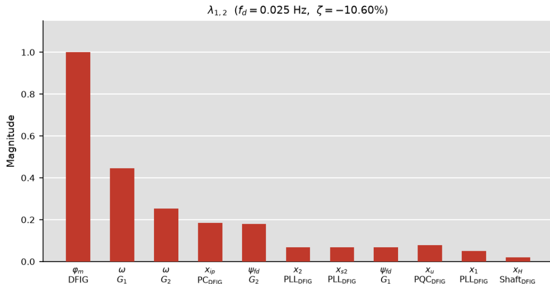
Gambar 4.16. Grafik Participation Factor Mode Dominan ( \lambda_{1,2} ) Skenario 4.1
