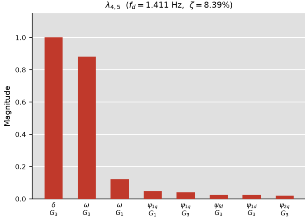
Gambar 4.22. Grafik Participation Factor Mode Dominan ( \lambda_{4,5} ) Skenario 5.2
