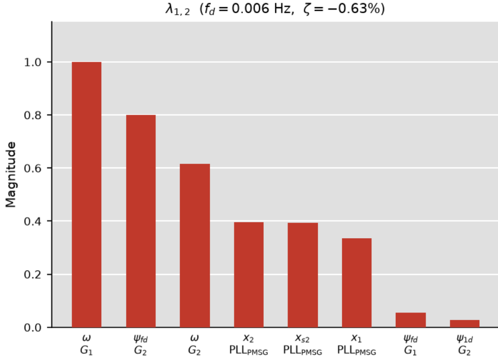
Gambar 4.20. Grafik Participation Factor Mode Dominan ( \lambda_{1,2} ) Skenario 5.1
