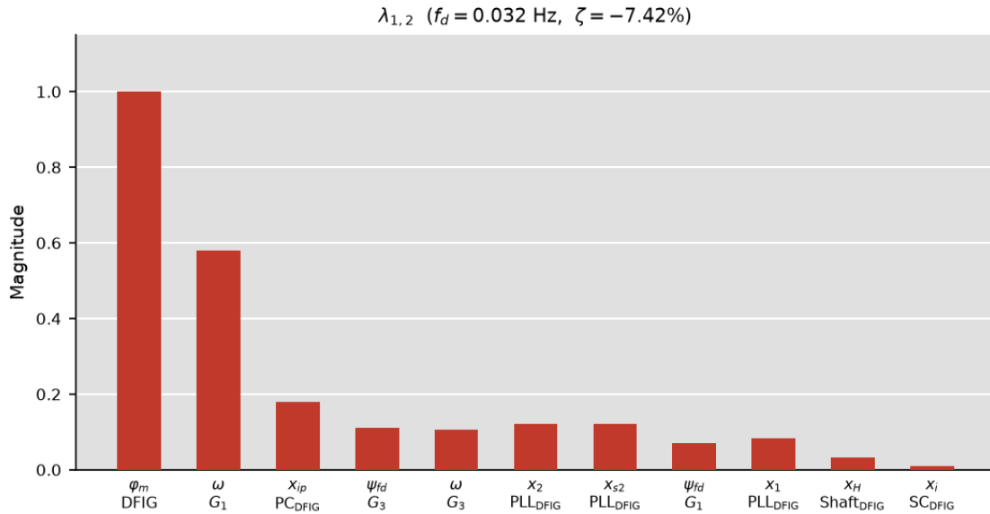
Gambar 4.18. Grafik Participation Factor Mode Dominan ( \lambda_{1,2} ) Skenario 4.2
