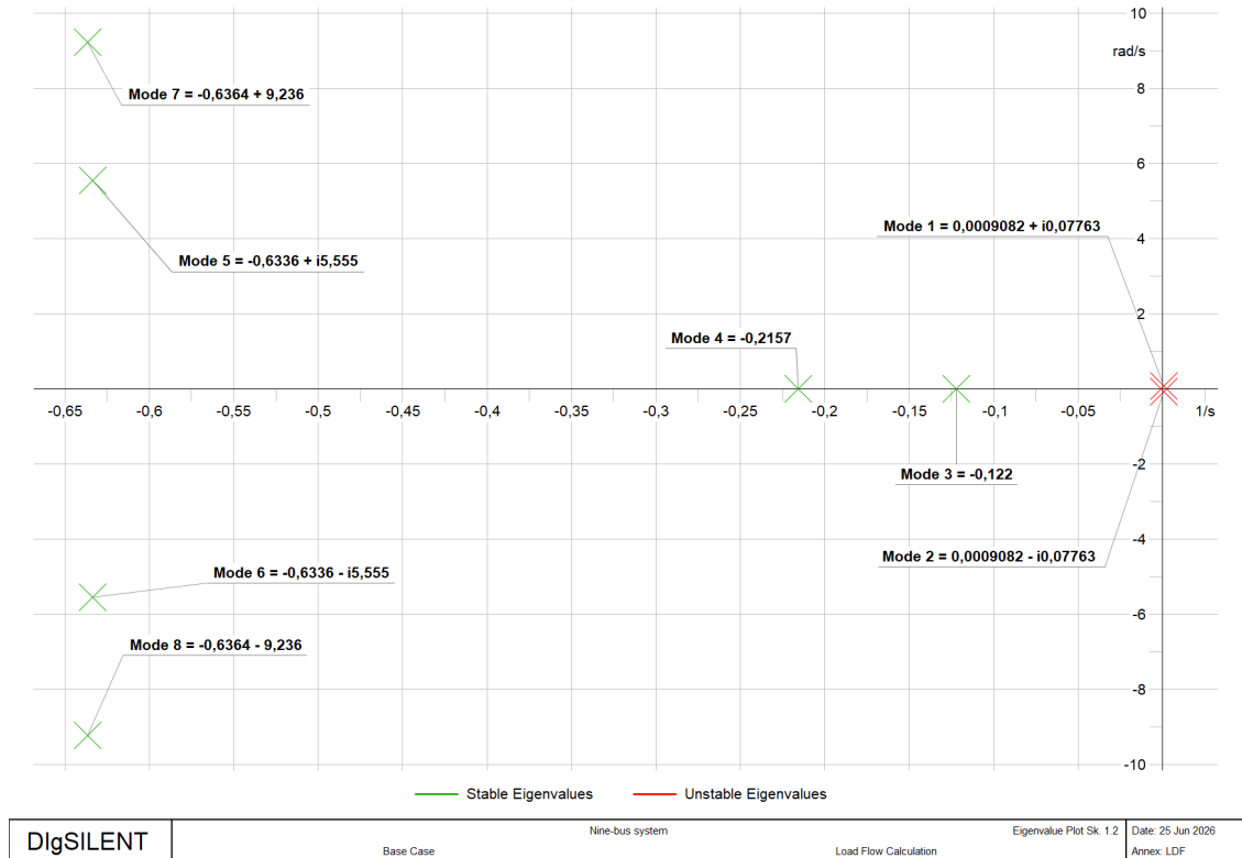
Gambar 4.3. Eigenvalue Plot Skenario 1.2
