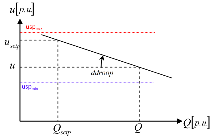
Figure 3.3: Voltage Q-Droop Control
