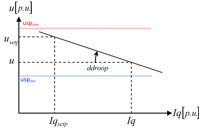
Figure 3.5: Voltage Iq-Droop Control
