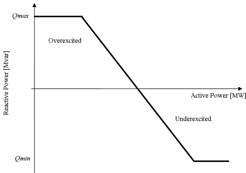
Figure 3.6: Q(P)-Characteristic
