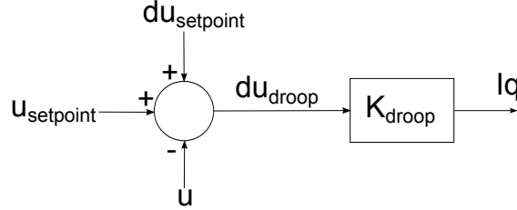
Figure 3.4: Voltage Iq-Droop Control
