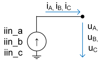
Figure 7.4: Current source model using phase currents as inputs
