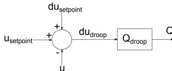
Figure 3.2: Voltage Q-Droop Control
