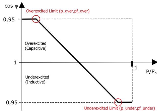
Figure 3.8: \cos\phi(P) -Characteristic: pf\_over < pf\_under
