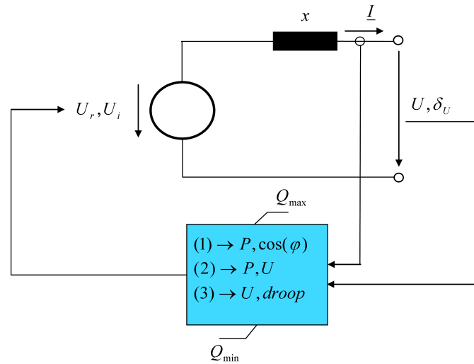
Figure 3.1: Local Controller - Options
