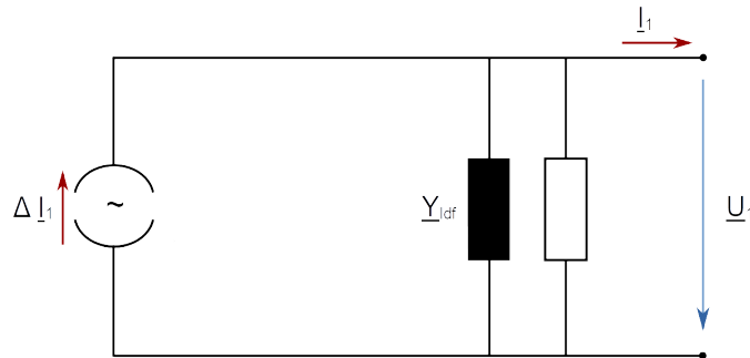
Figure 4.3: Equivalent positive sequence circuit for constant current injections used in the complete short-circuit calculation
