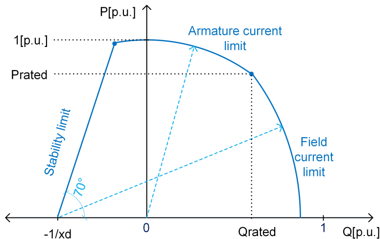
Figure 2.7: Base capability curve of the synchronous machine
