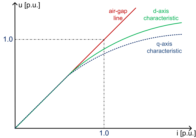
Figure 6.6: d- and q-axis saturation characteristics
