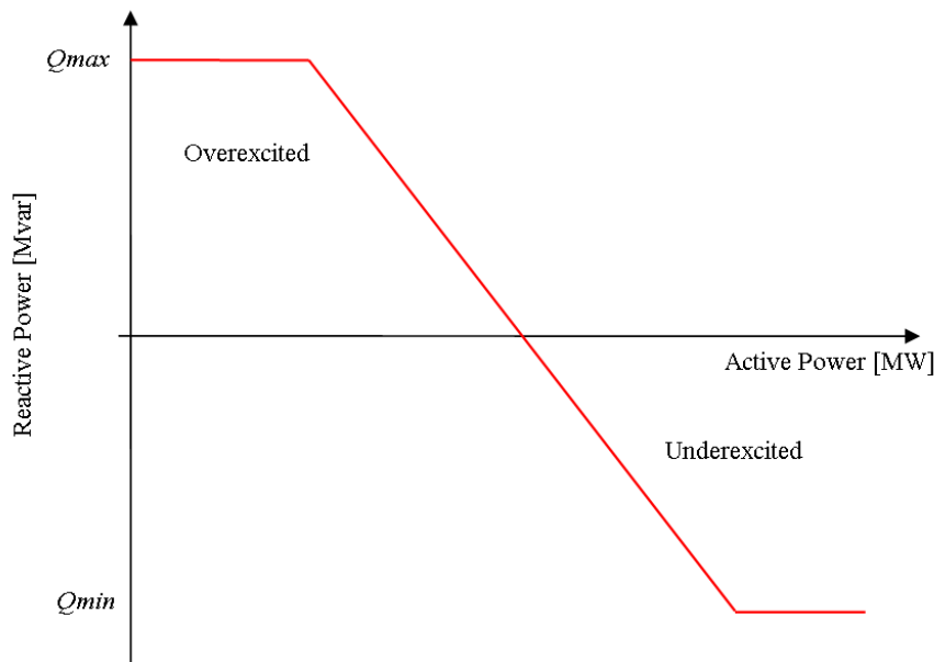
Figure 2.6: Q(P)-Characteristic
