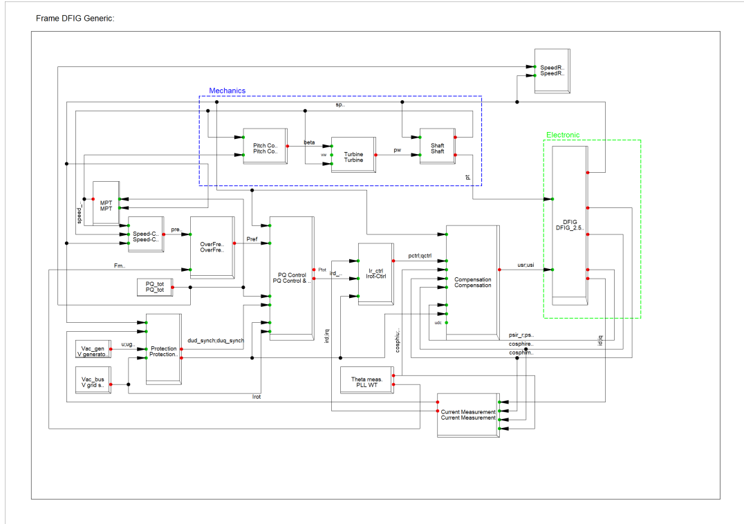
Gambar 3.3. Model Kontrol Komposit DFIG-WT [26]
