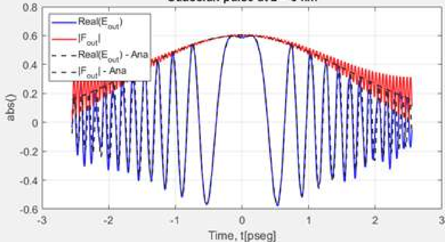
Gaussian pulse at z = 3 km
