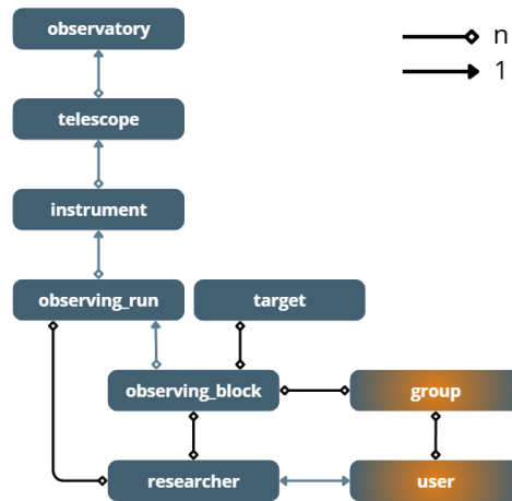
Figure II.3. Database structure and relationships between tables.
