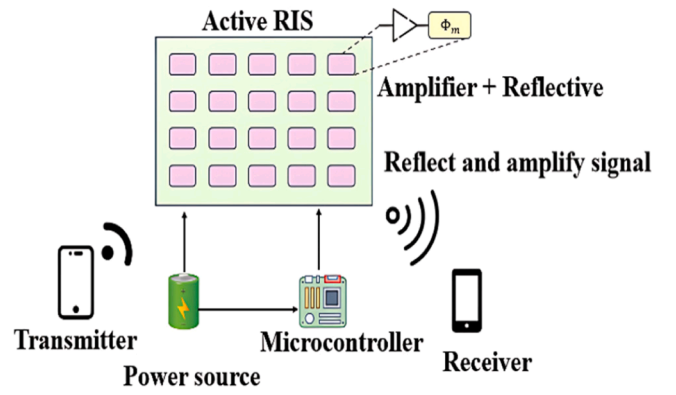
Fig. 4. A scheme of the active RIS.
