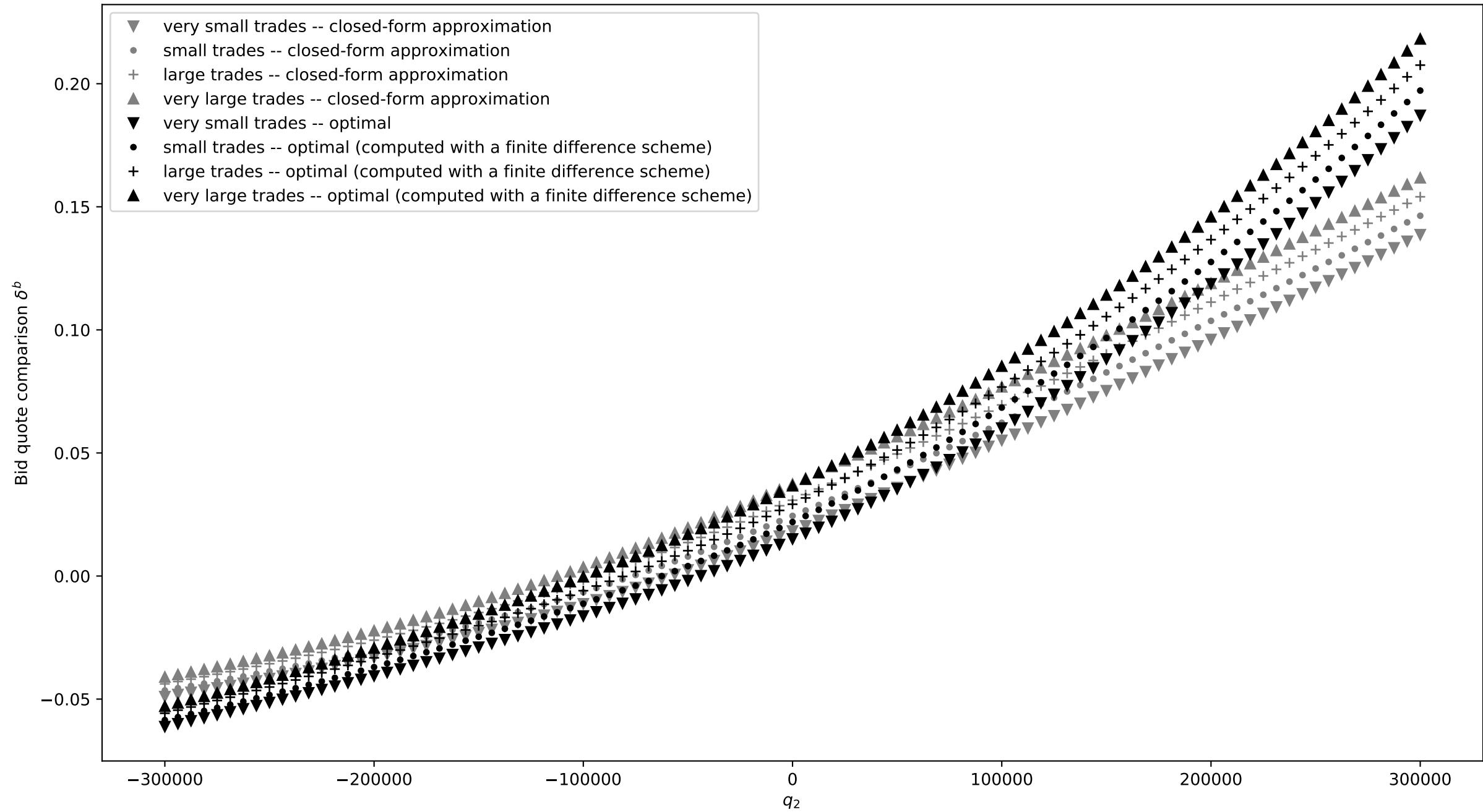
Comparison of bid quotes for asset 1 for different trade sizes as a function of q_2 ( q_1 = 0 )
