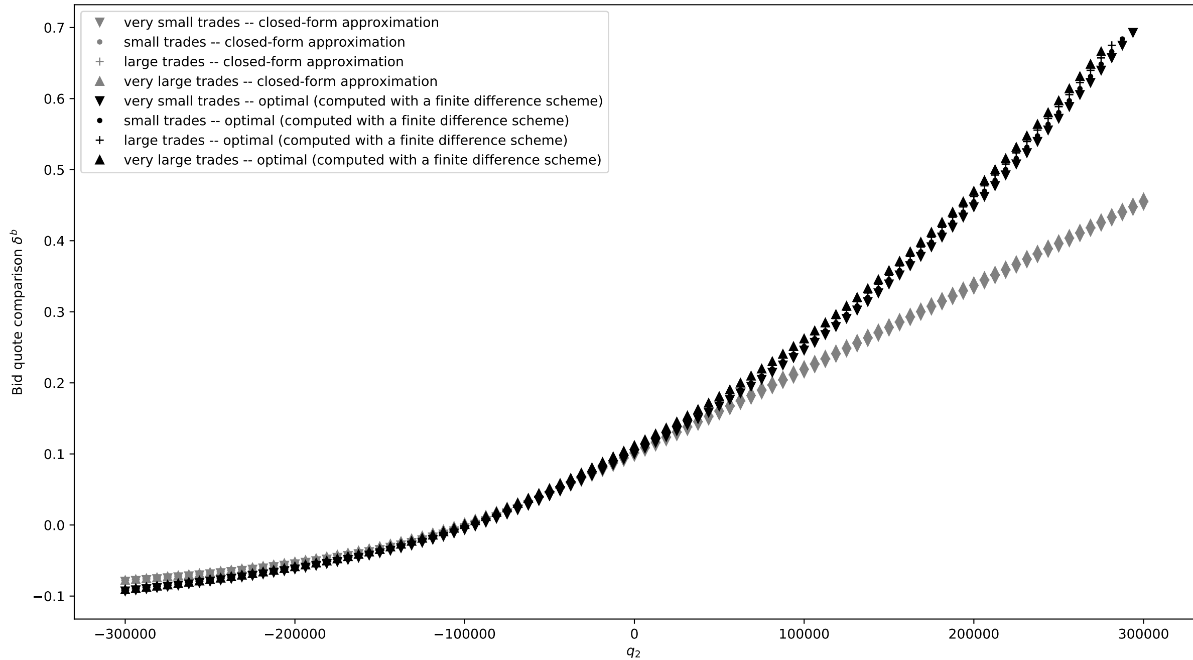
Comparison of bid quotes for asset 2 for different trade sizes as a function of q_2 ( q_1 = 0 )
