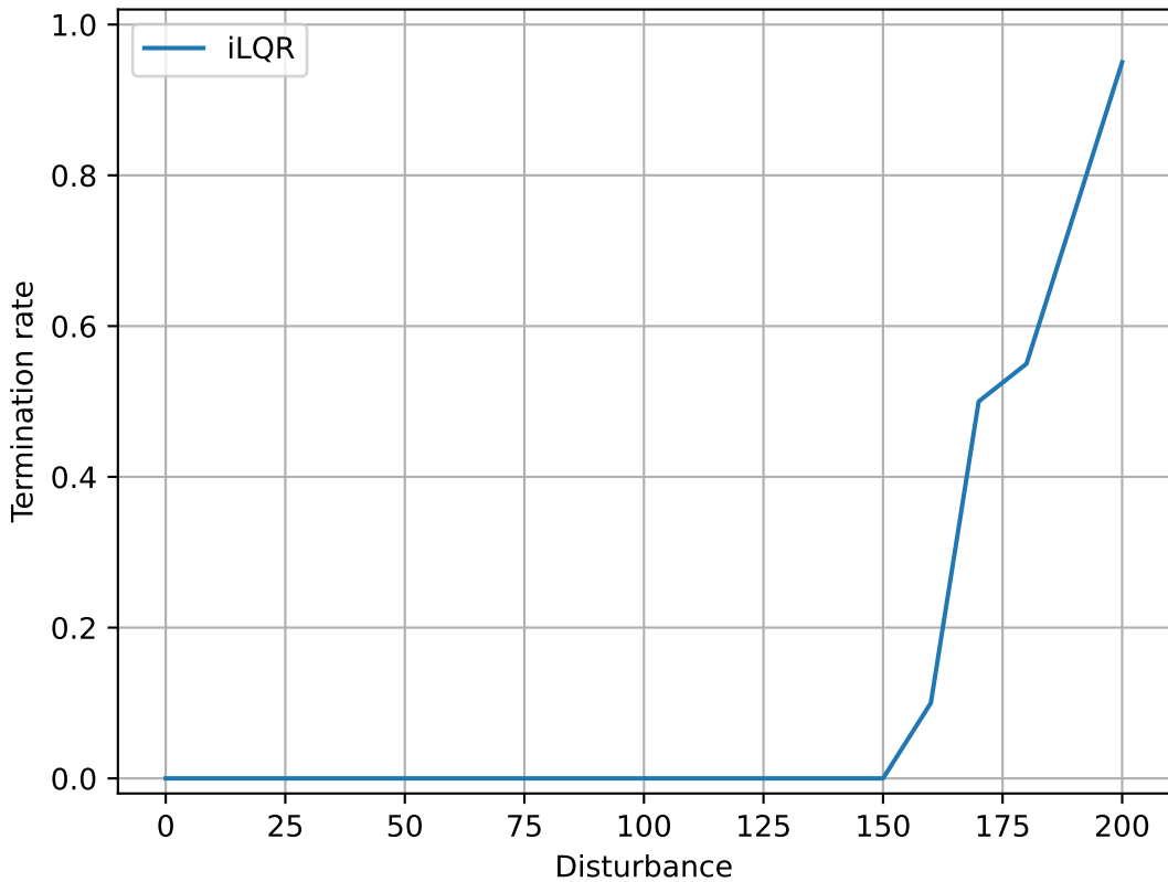
Termination rate vs disturbance - iLQR
