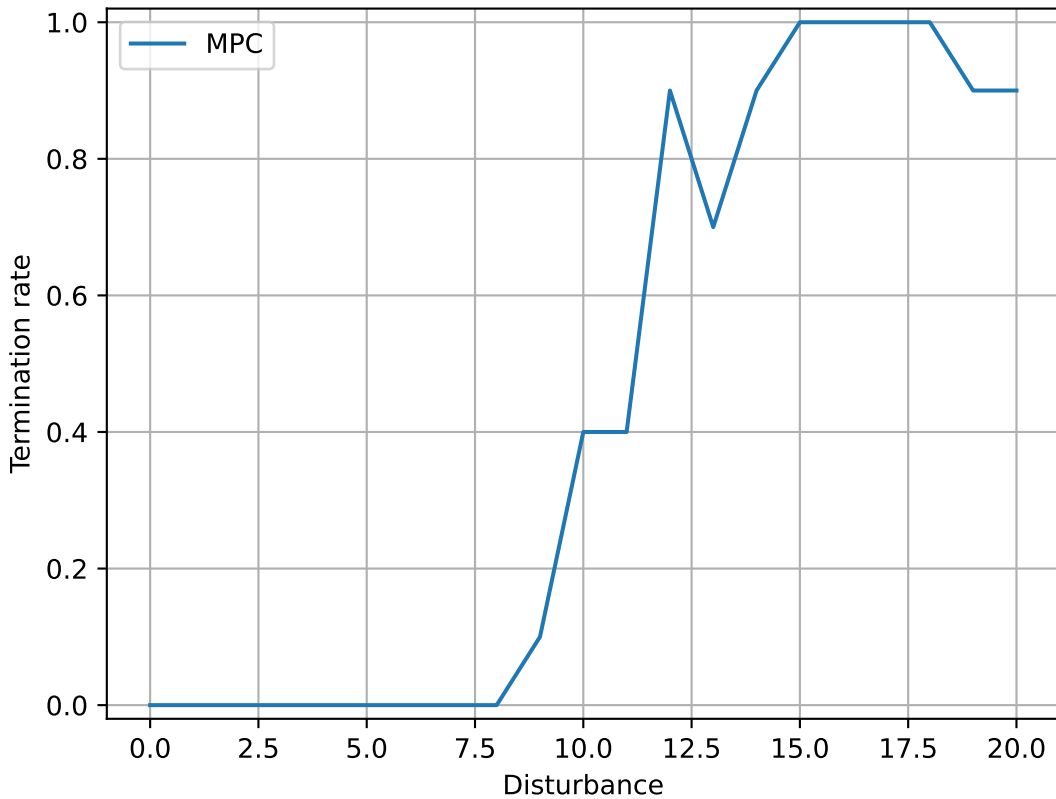
Termination rate vs disturbance - MPC
