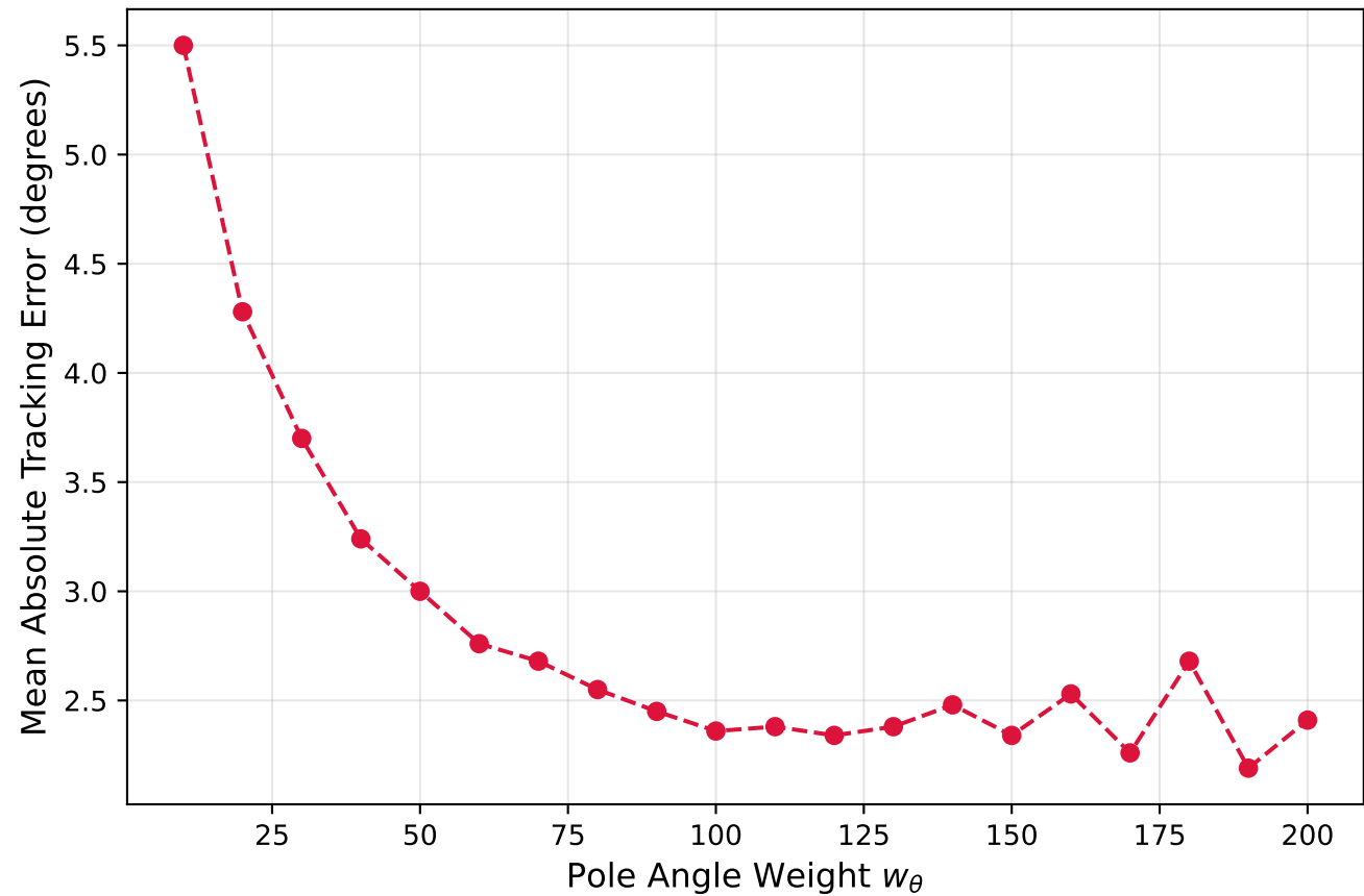
Angle Tracking Performance vs w_\theta
