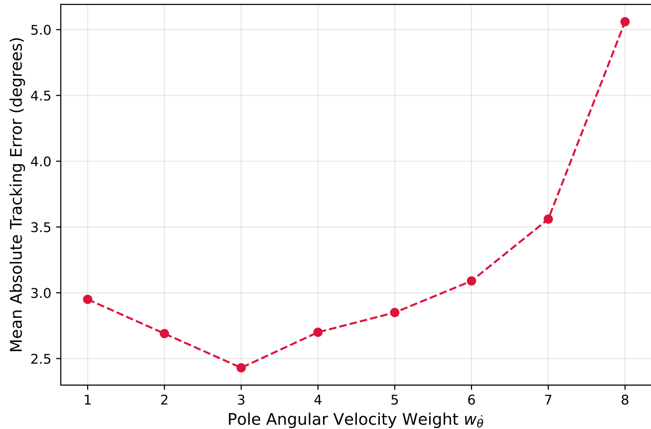
Angle Tracking Performance vs w_{\dot{\theta}}
