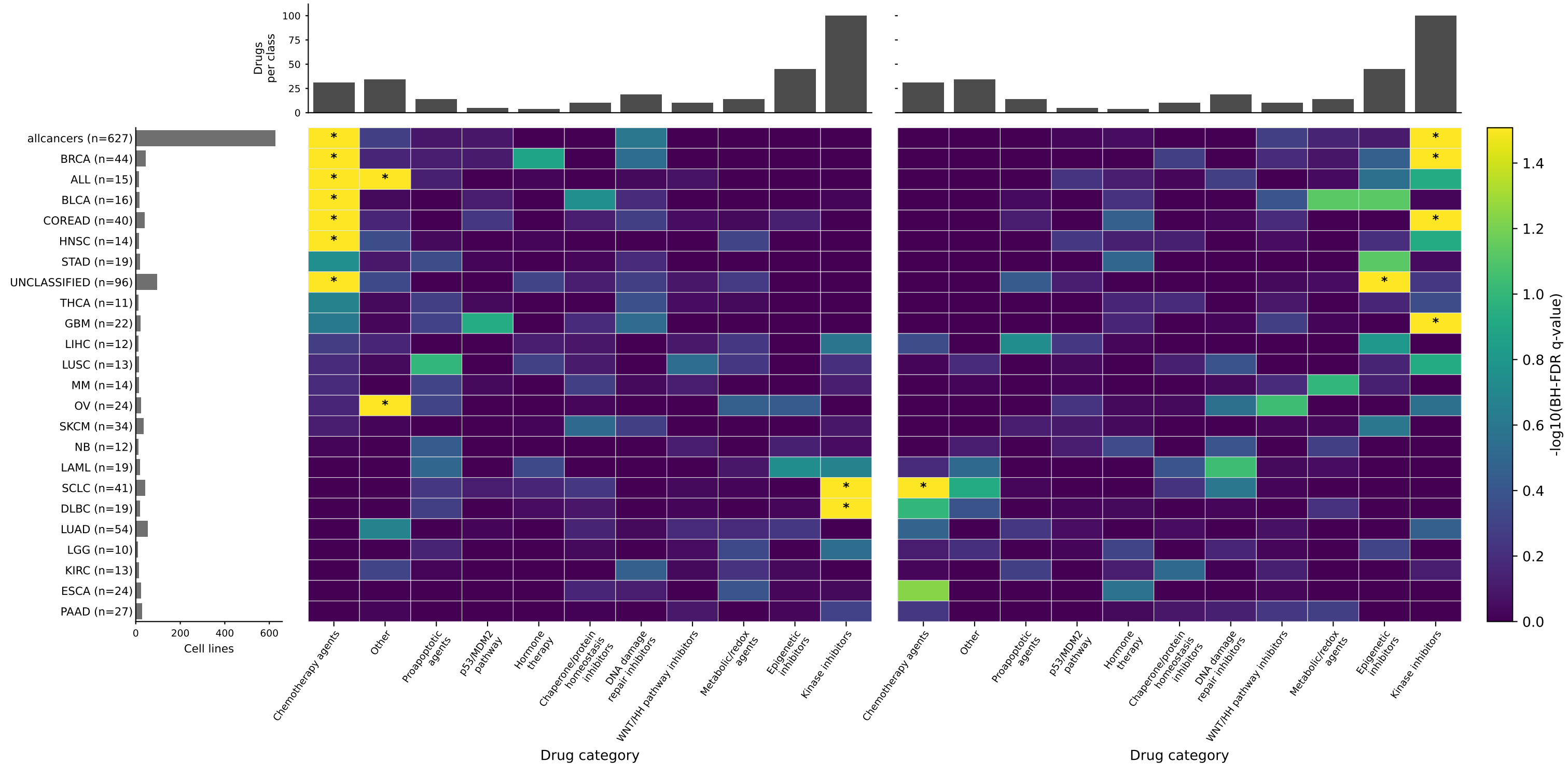
Low-ploidy-selective enrichment (ordered by chemotherapy-agent FDR significance)
