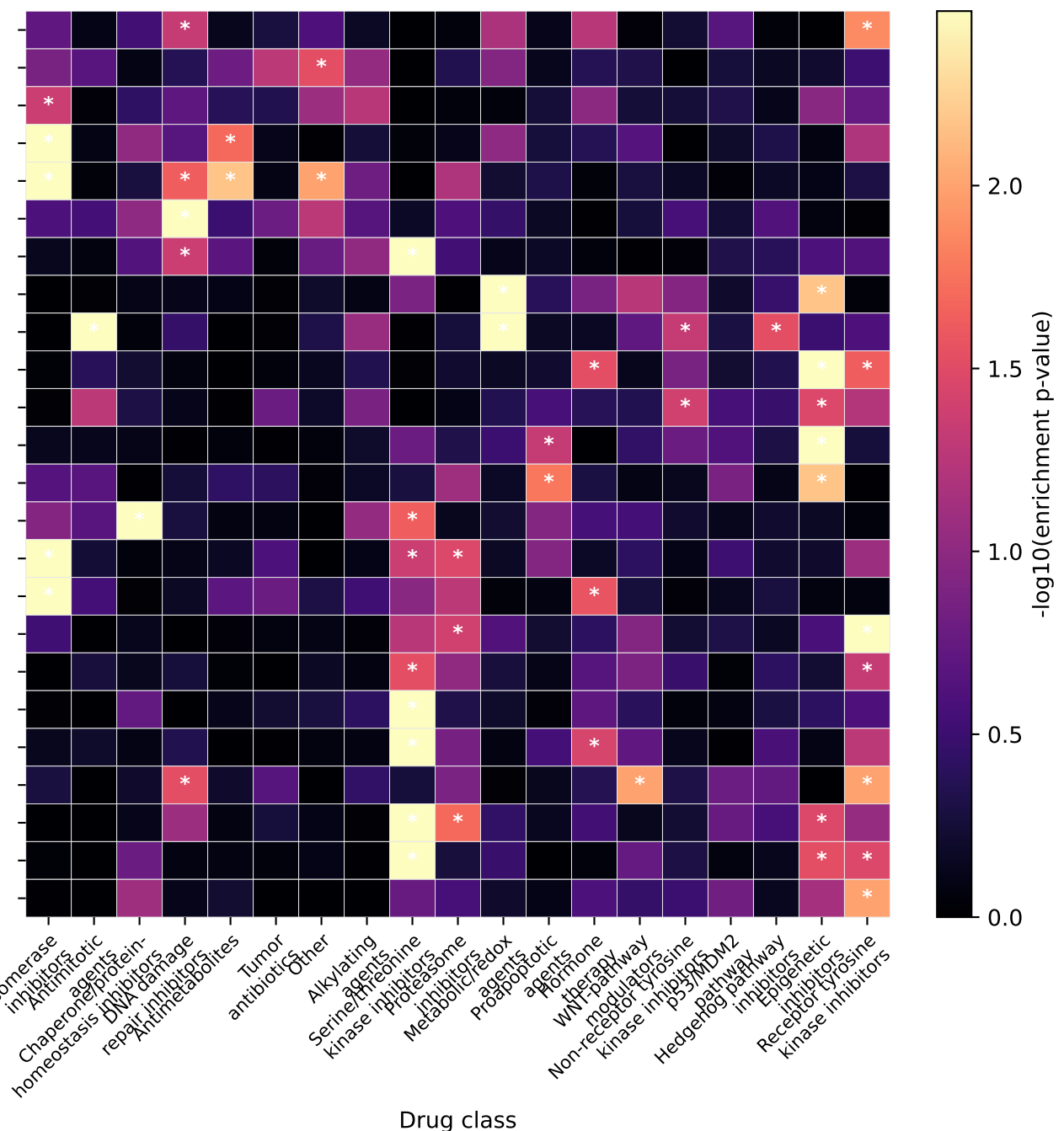
High-ploidy-selective enrichment
