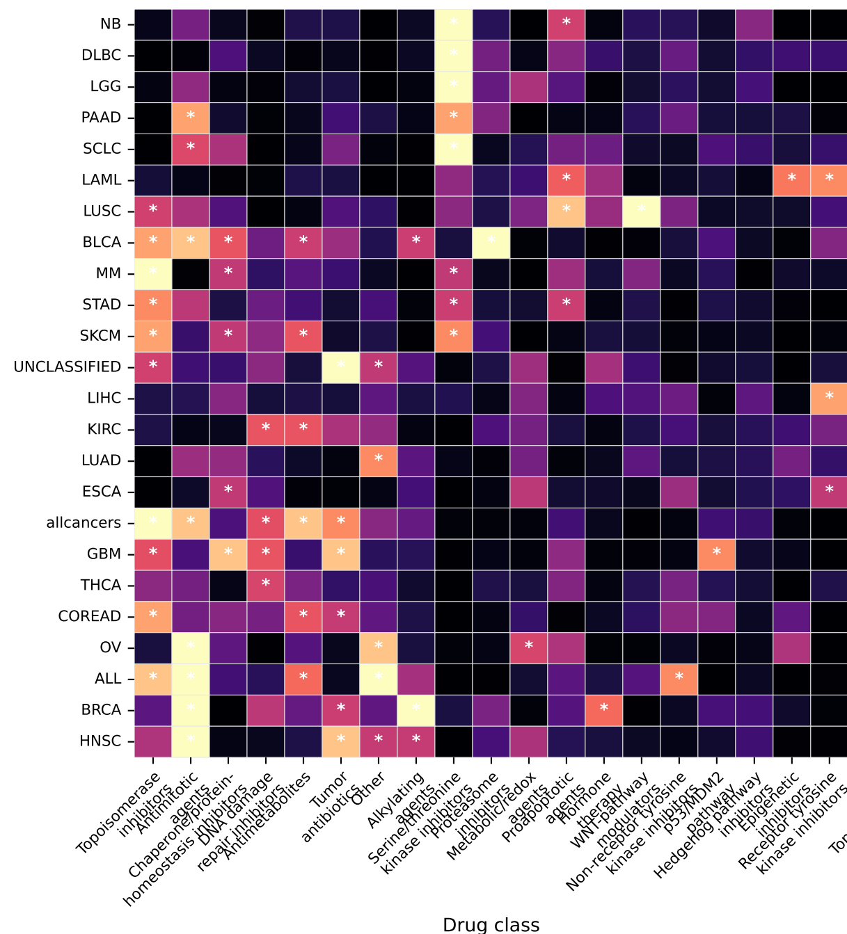
Low-ploidy-selective enrichment
