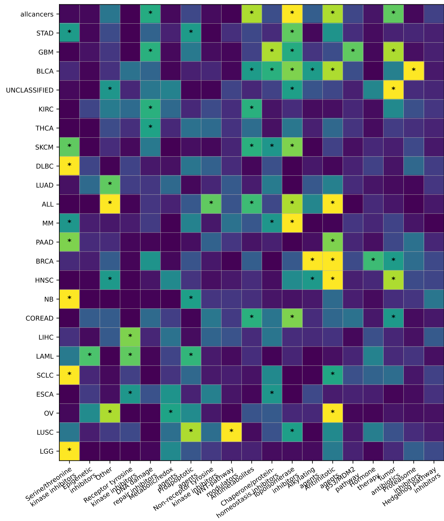
Low-ploidy-selective enrichment
