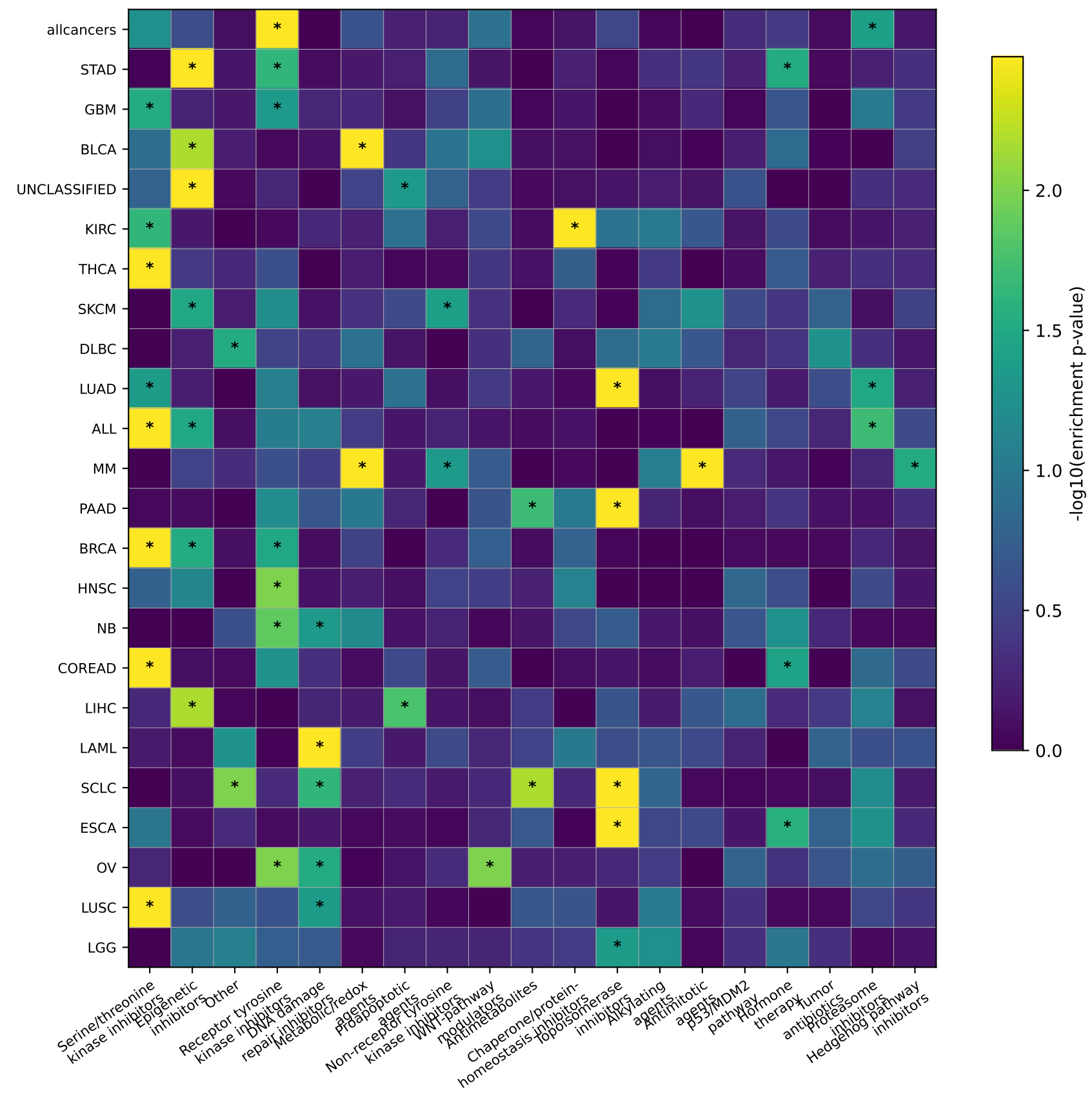
High-ploidy-selective enrichment
