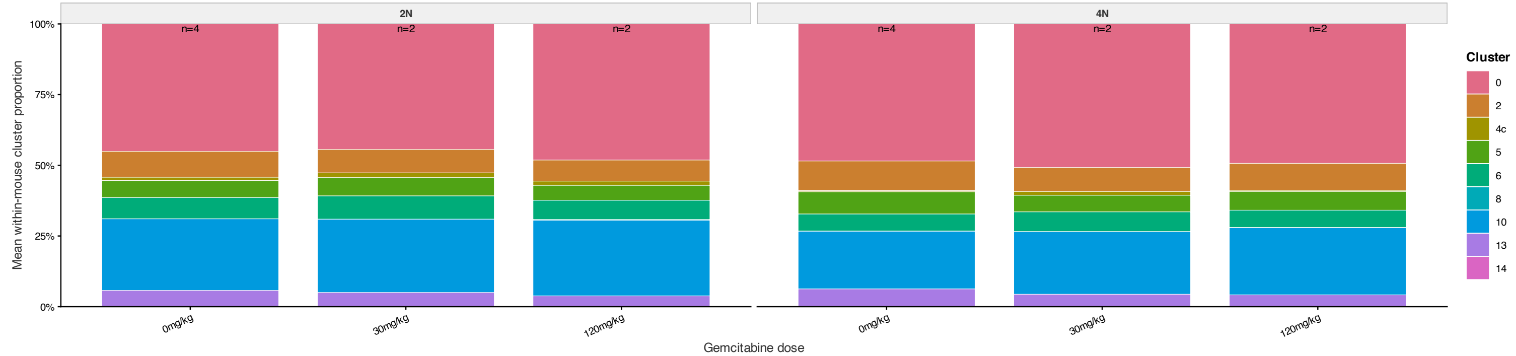
G Equal-mouse composition by initial ploidy and dose Within-mouse proportions are averaged with equal mouse weights; stars mark dose enrichment within ploidy at BH FDR <= 0.05
