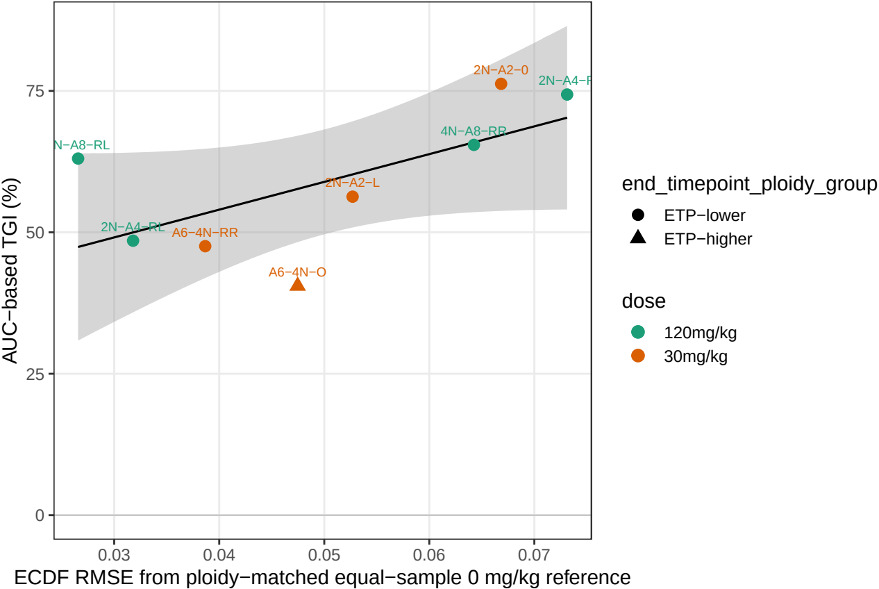
Cell-cycle-associated tumor cells: AUC TGI vs sample-equal ECDF shift
