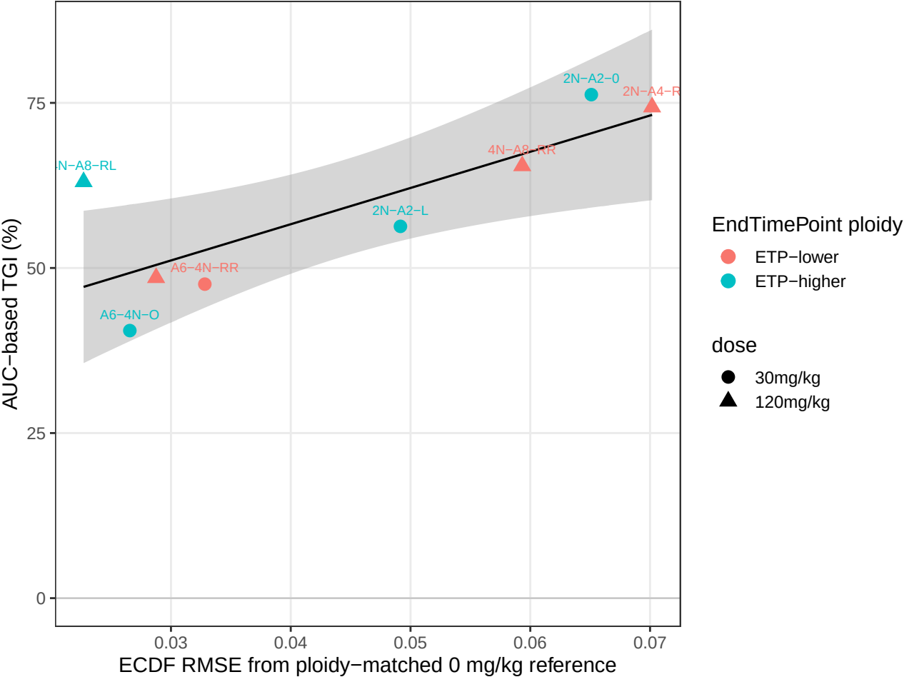
CellCycle: AUC-TGI association with pseudotime shift and ploidy
