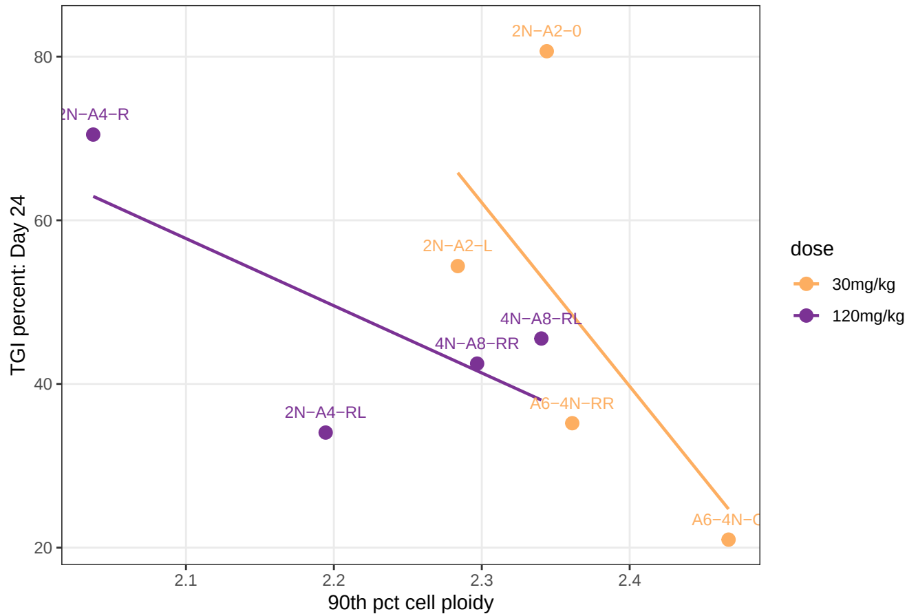
Day 24 TGI versus 90th-percentile ploidy in treated samples
