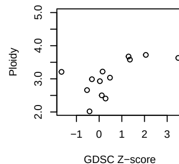
BLCA Romidepsin
