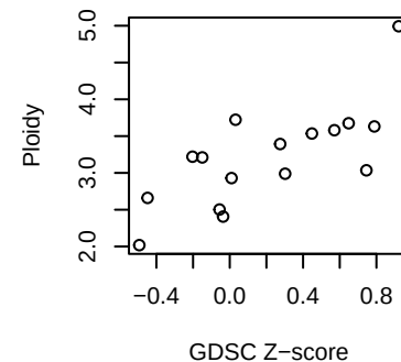
BLCA Motesanib
