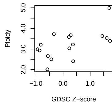
BLCA ZM447439
