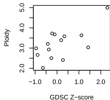
BLCA PBD-288
