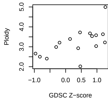
BLCA KU-55933
