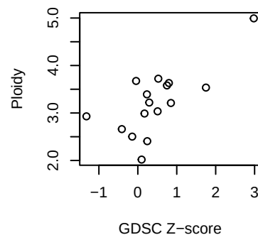
BLCA Pictilisib
