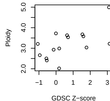
BLCA Mirin
