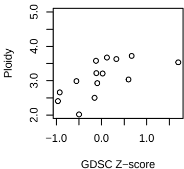
BLCA GSK2606414
