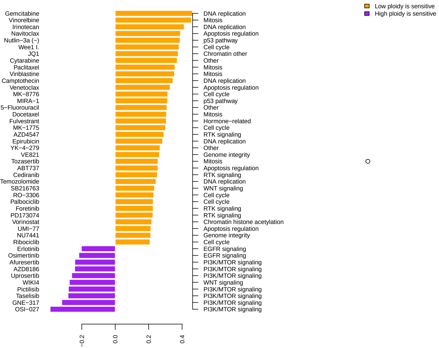
Pearson r(ploidy, drug-resistance Z-score)
