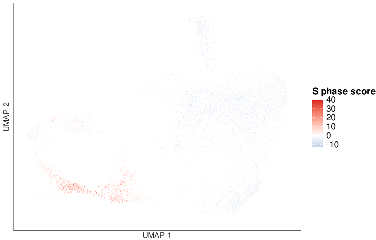
D UMAP by S phase score
