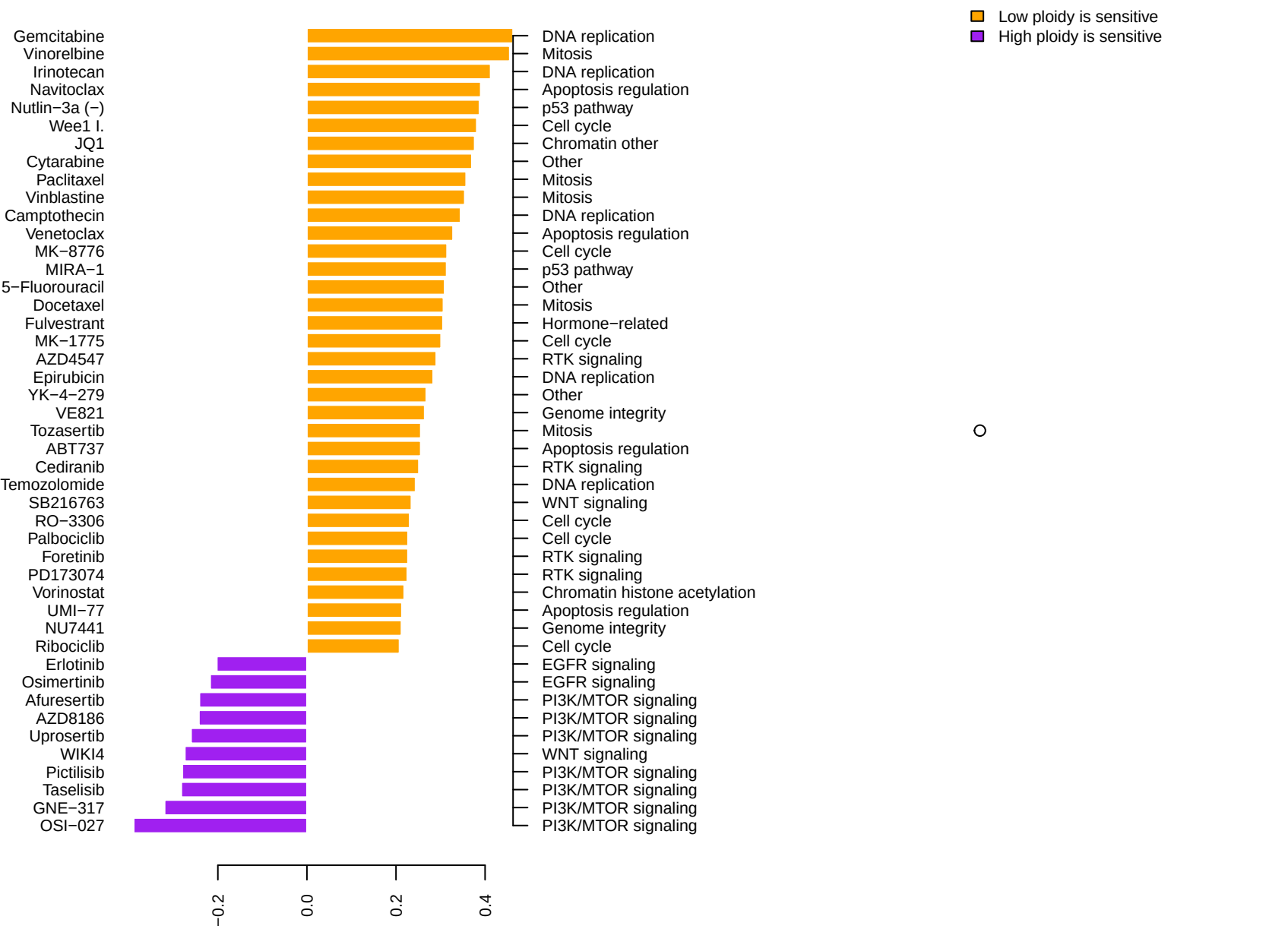
Pearson (ploidy, BreastCancerDrugSensitivity Z Score)
