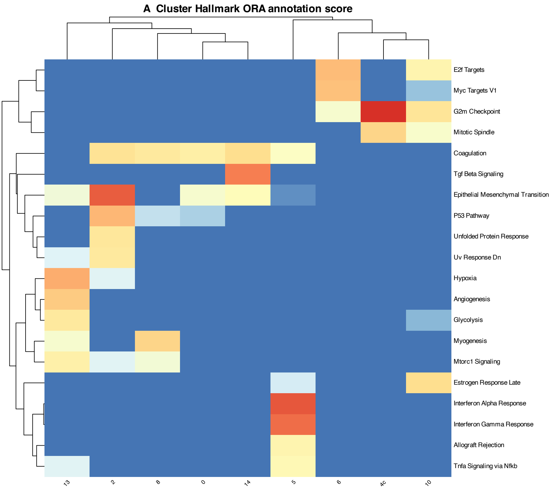
Supplementary Figure 7 | Cluster Hallmark pathway analysis
