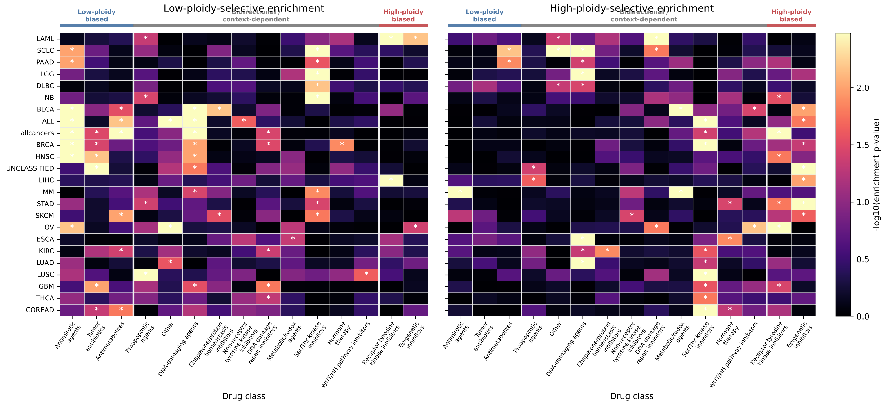
GDSC ploidy-enrichment heatmaps ordered by collapsed drug-class direction
