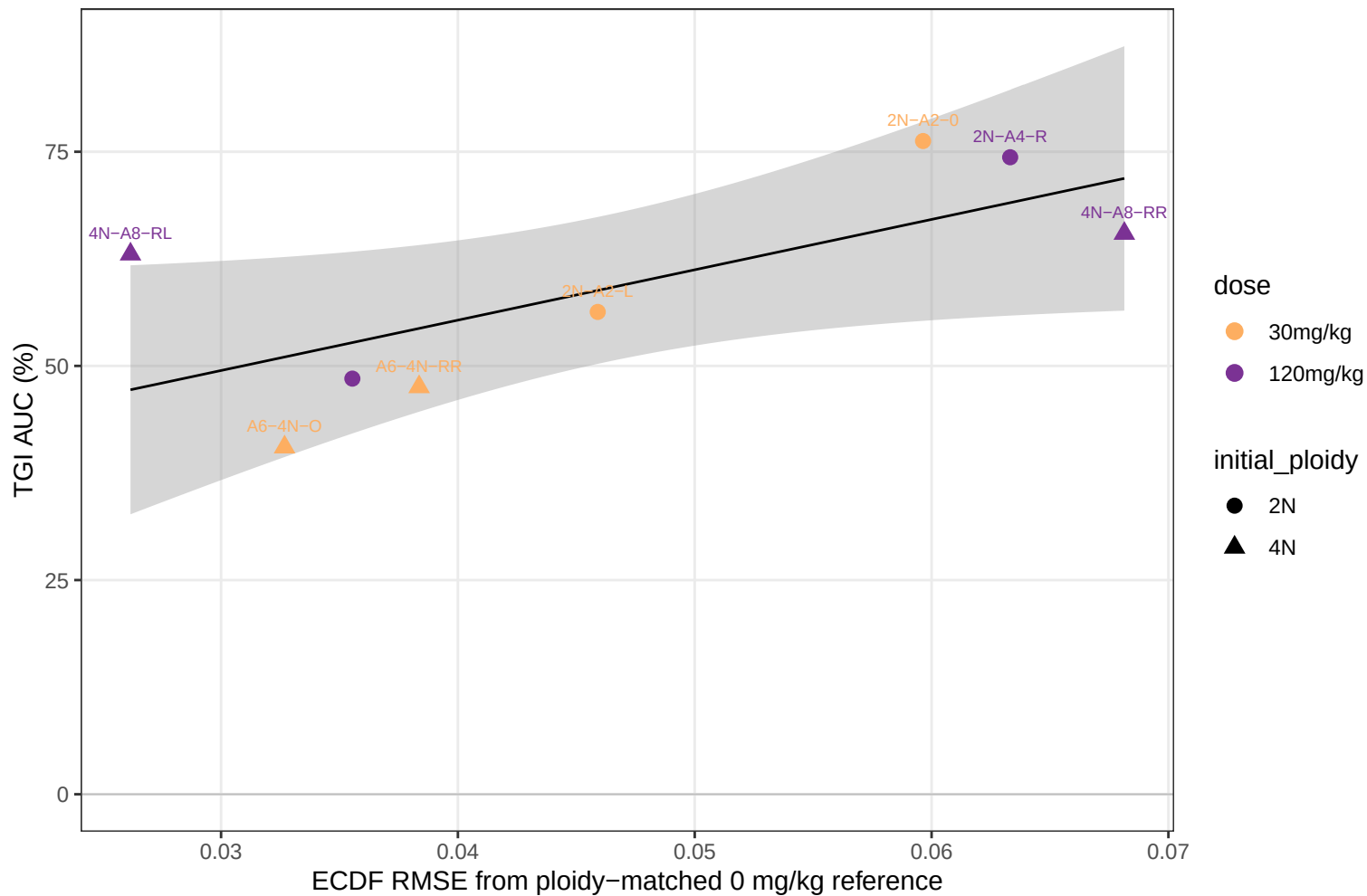
TGI AUC versus pseudotime distance from ploidy-matched controls
