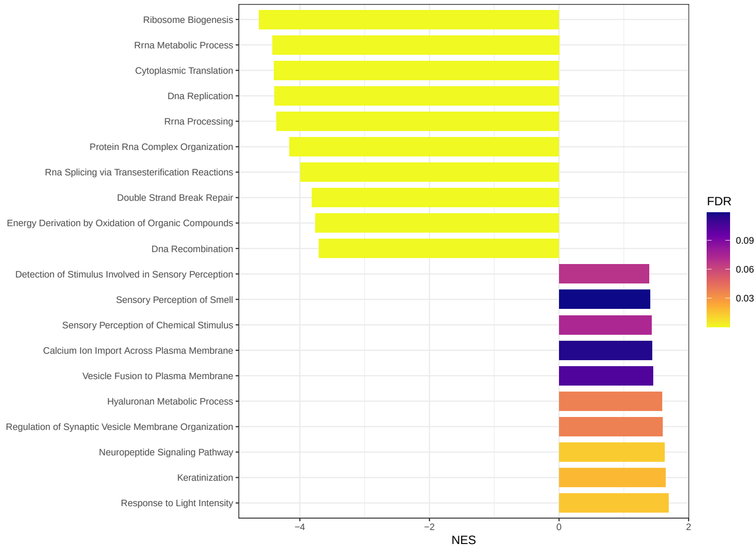
ETP_boundary_stress_threshold_2_375: go_bp GSEA
