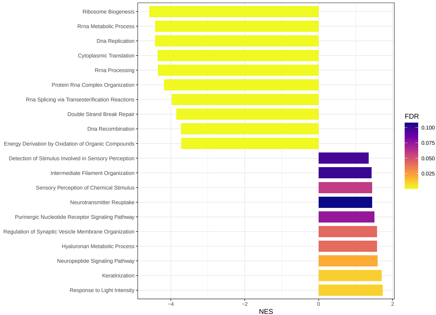
ETP_reference_balanced_threshold_2_24: go_bp GSEA
