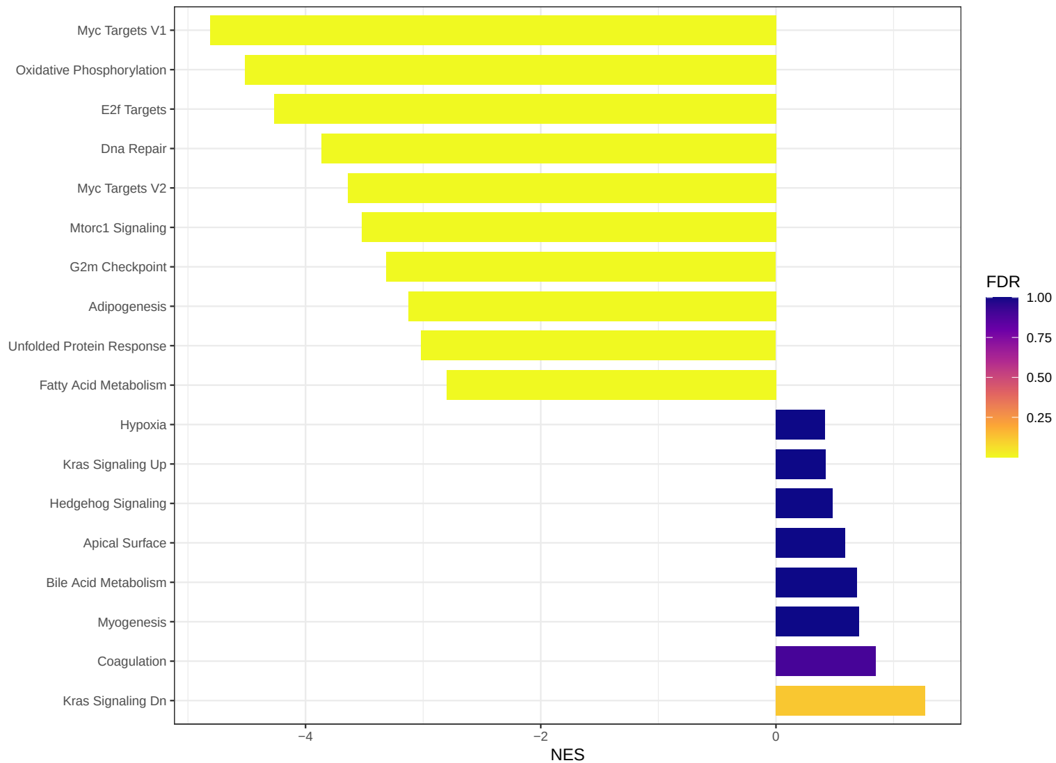
ETP_reference_balanced_threshold_2_24: hallmark GSEA
