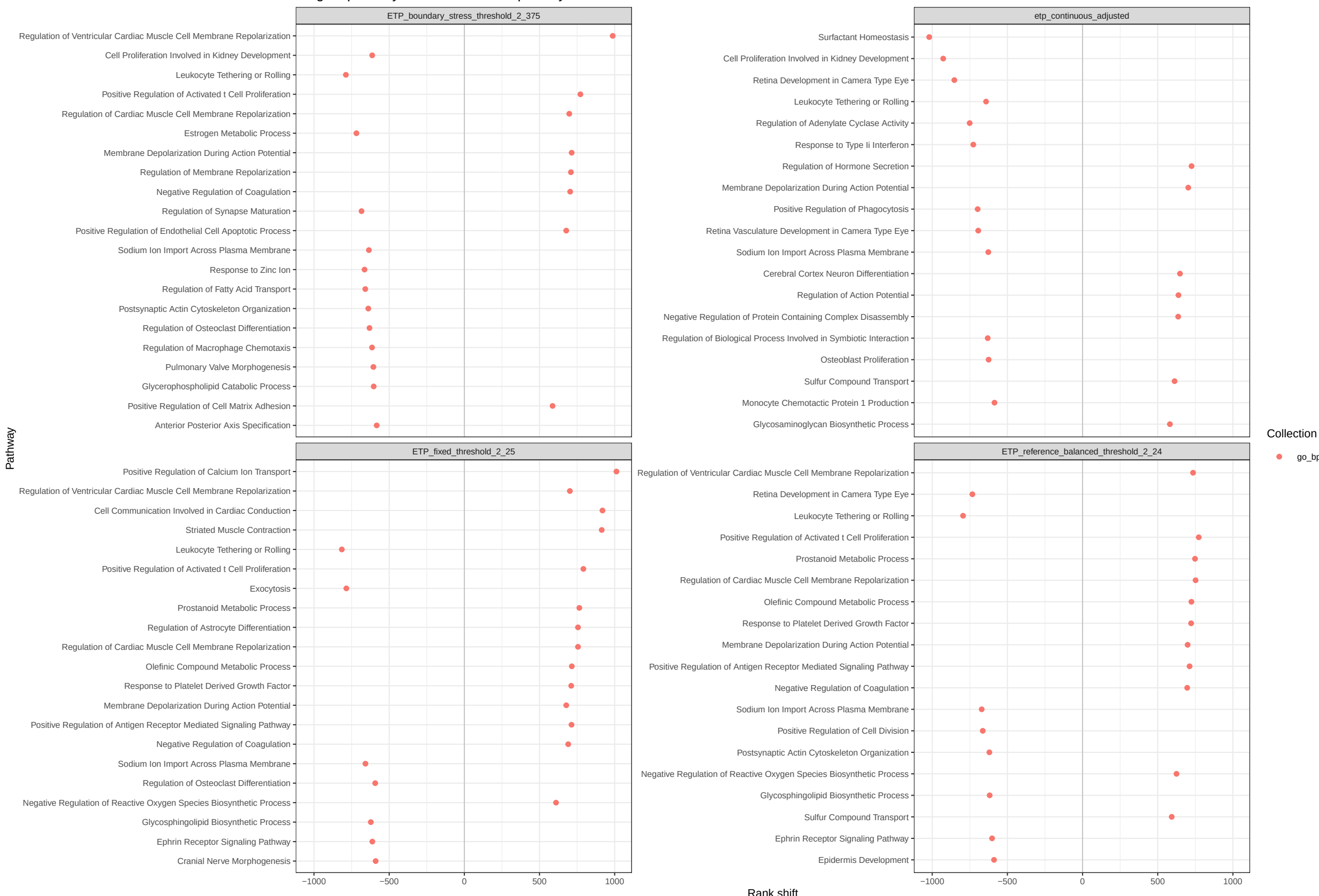
Largest pathway rank shifts versus primary model
