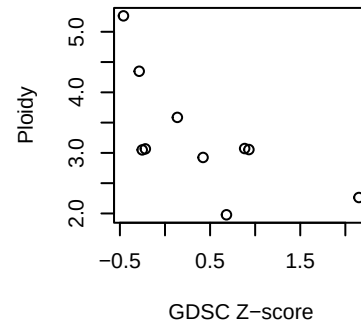
LGG SB216763
