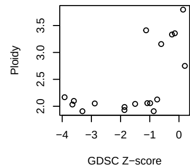
LAML Venetoclax
