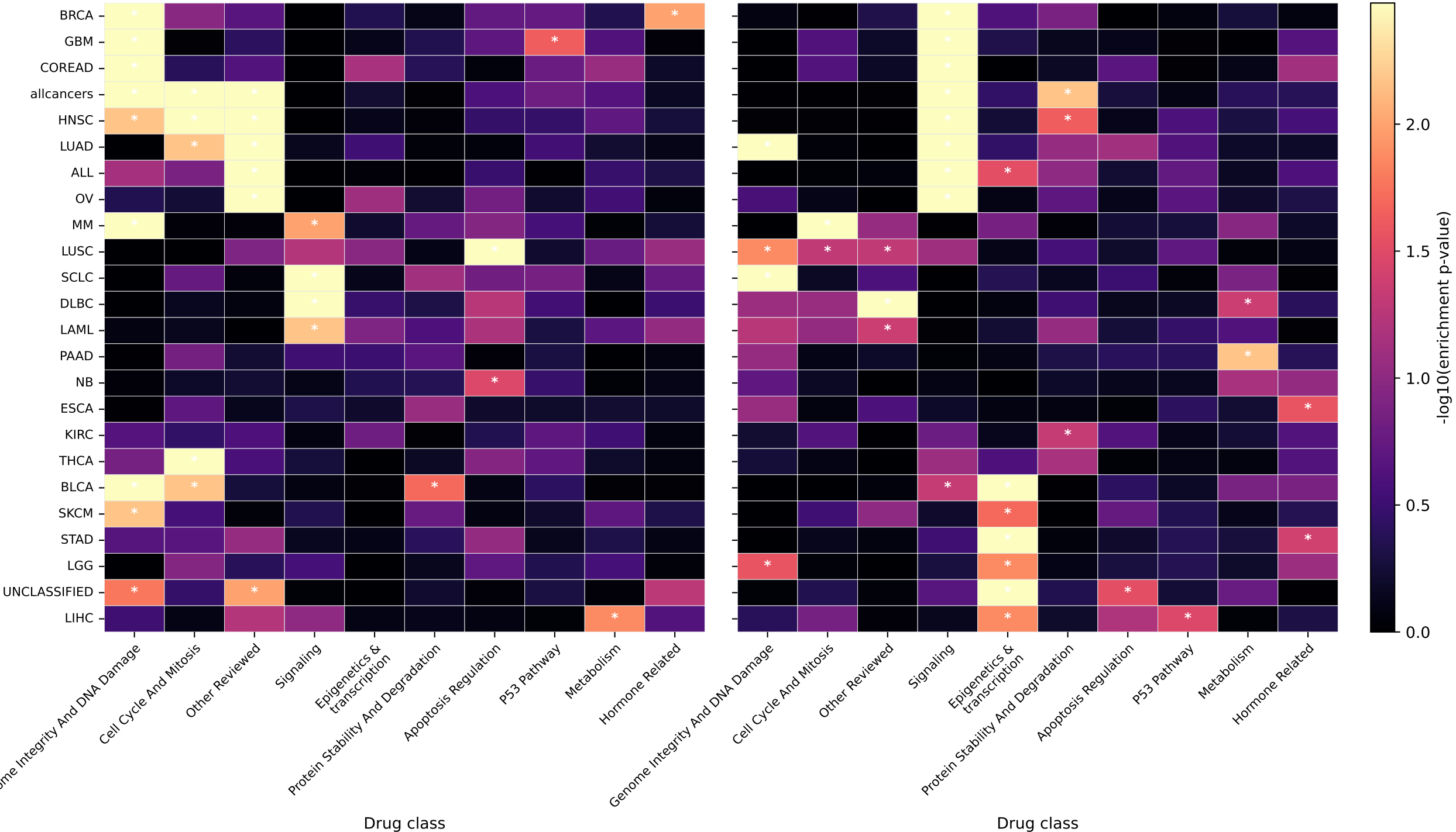
Low-ploidy-selective enrichment
