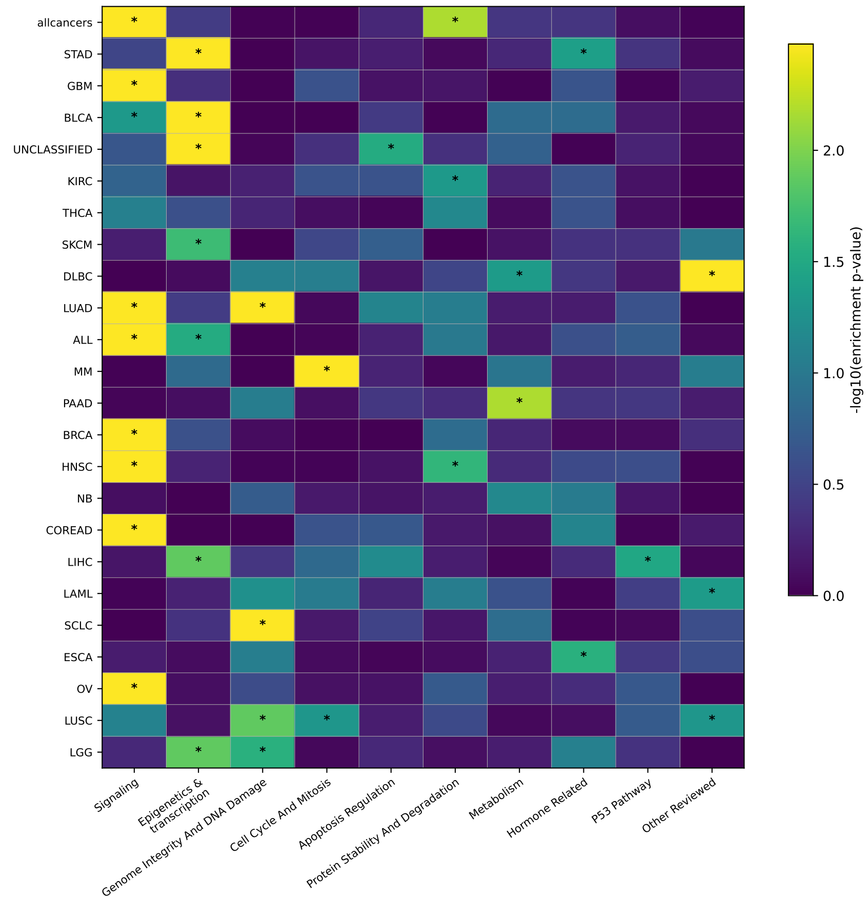
High-ploidy-selective enrichment
