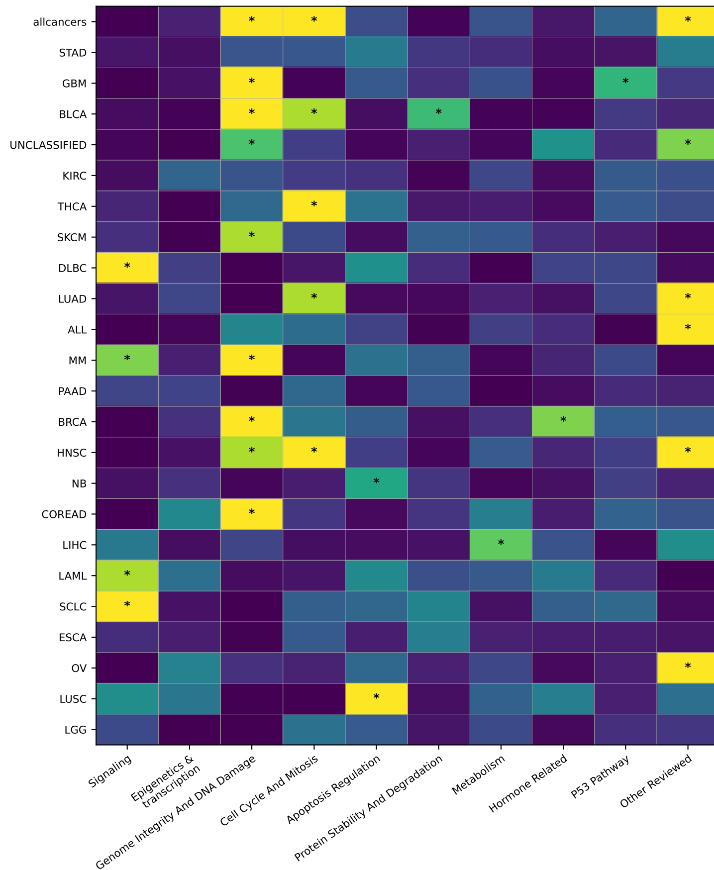
Low-ploidy-selective enrichment
