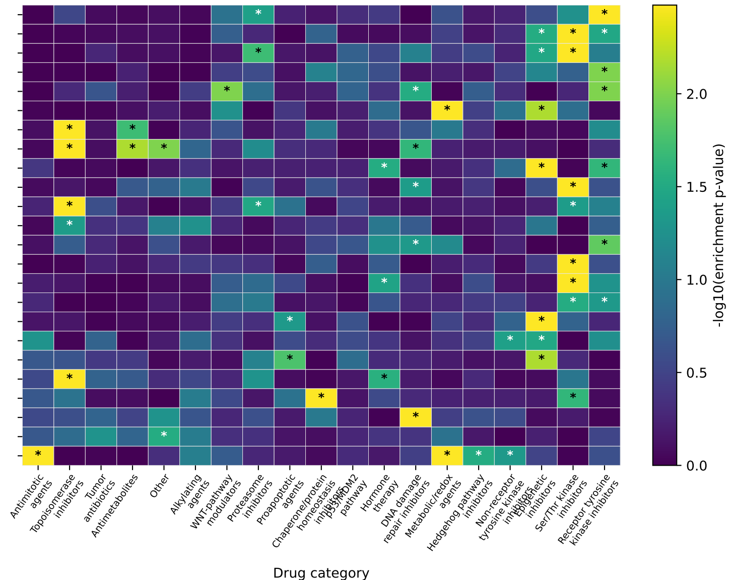
High-ploidy-selective enrichment (same row and drug-class order)
