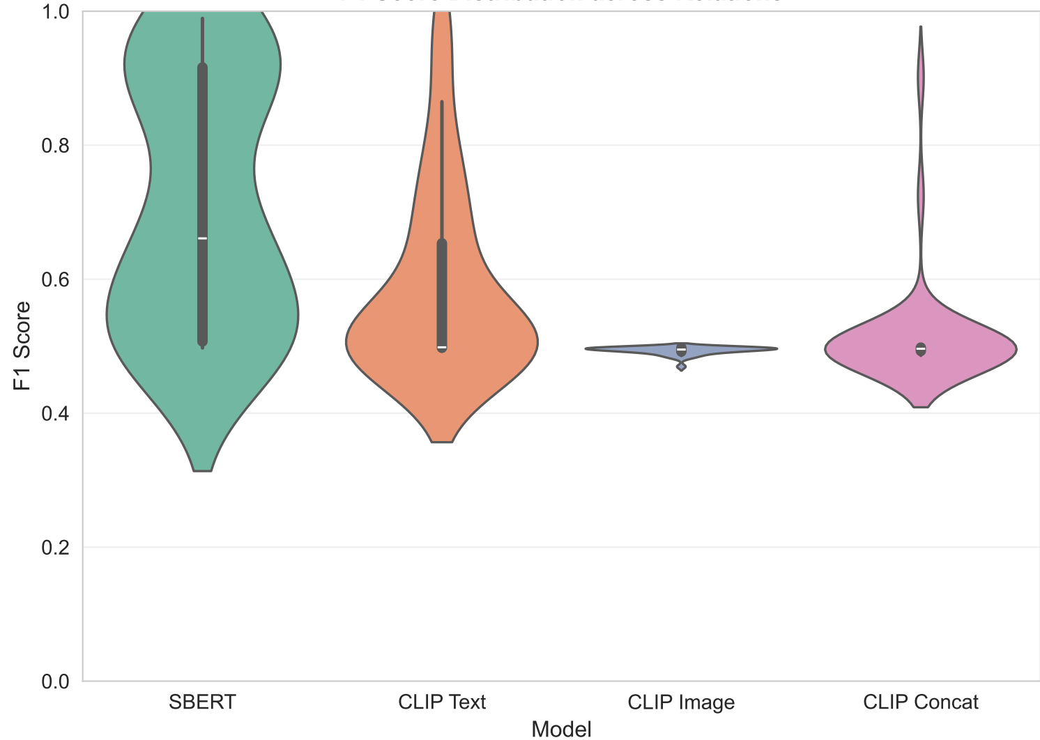
F1 Score Distribution across Relations
