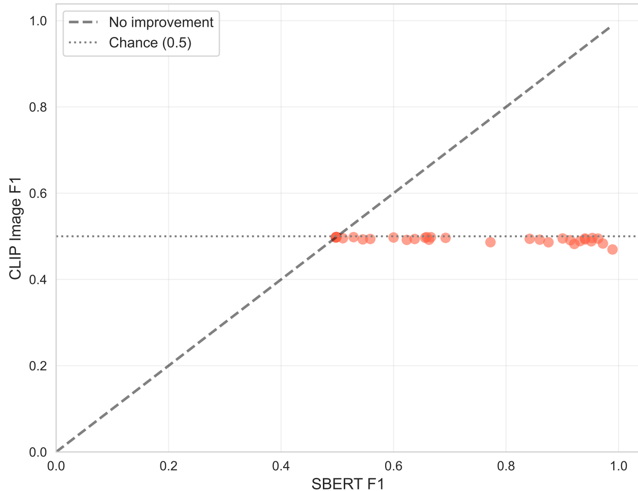
CLIP Image vs SBERT (pooled image encoder — null result)
