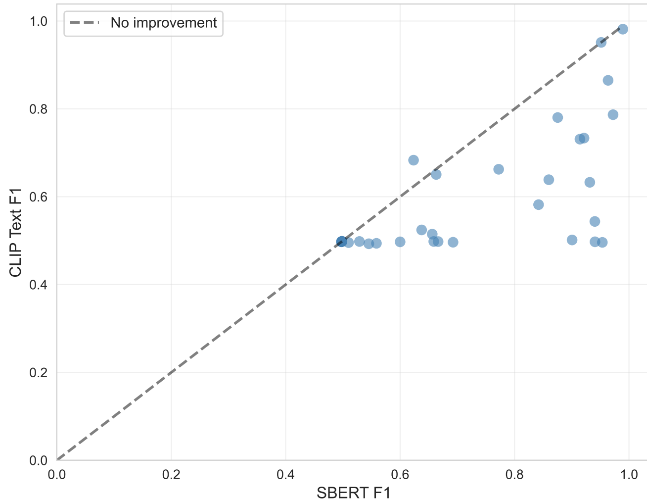
CLIP Text vs SBERT (text-encoder comparison)
