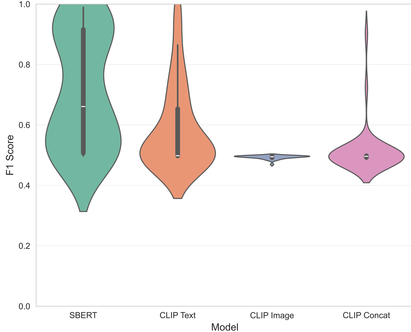
F1 Score Distribution across Relations
