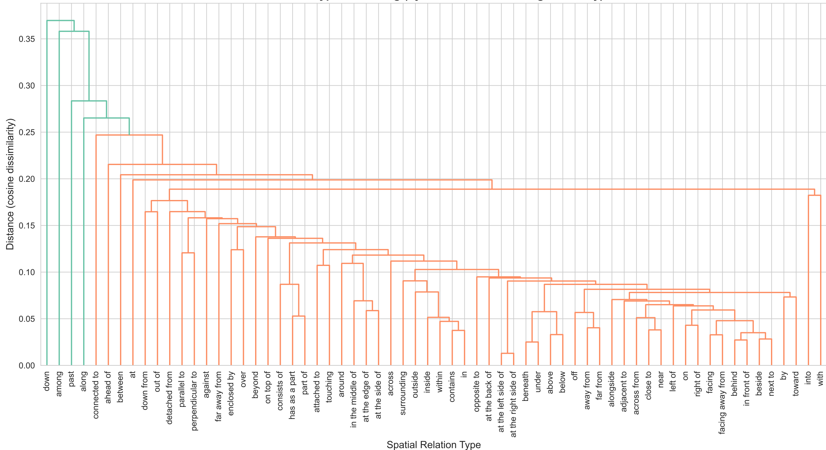
Relation Type Clustering (by CLIP Text Embedding Similarity)
