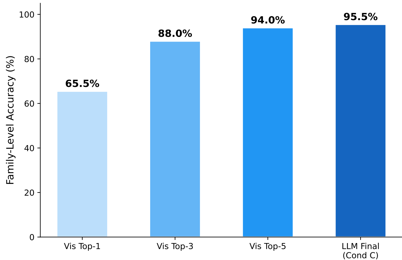
Visual Classifier Top-k vs LLM Rank Selection
