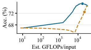
gRefCOCO / Q
