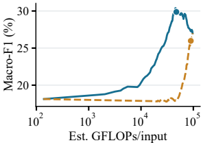
Construction / Q
