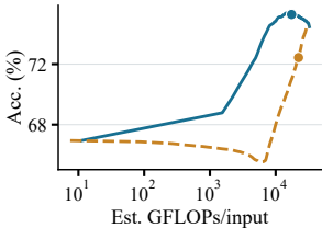
gRefCOCO / Q
