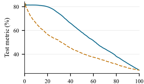
cub / ResNet
