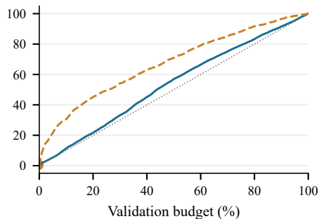
nlvr2 / ViLT
