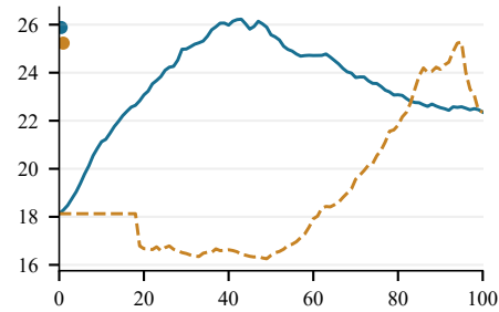
construction / YOLO26x
