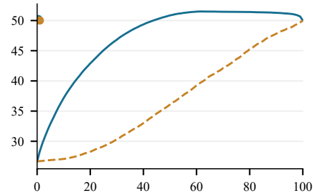
grefcoco / GroundingDINO
