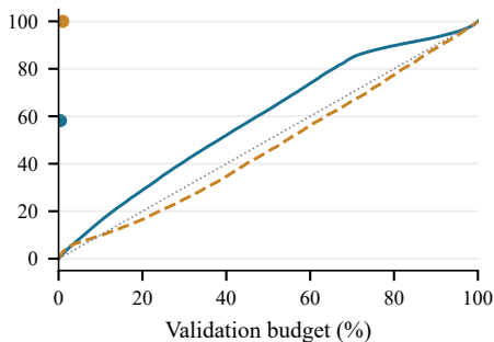
construction / YOLO26x
