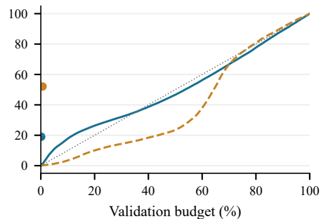
construction / RT-DETR-X
