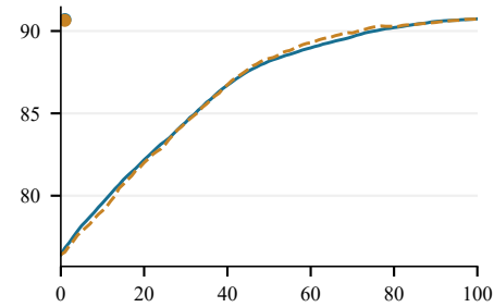
nlvr2 / ViLT
