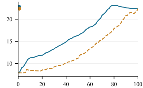
construction / RT-DETR-X
