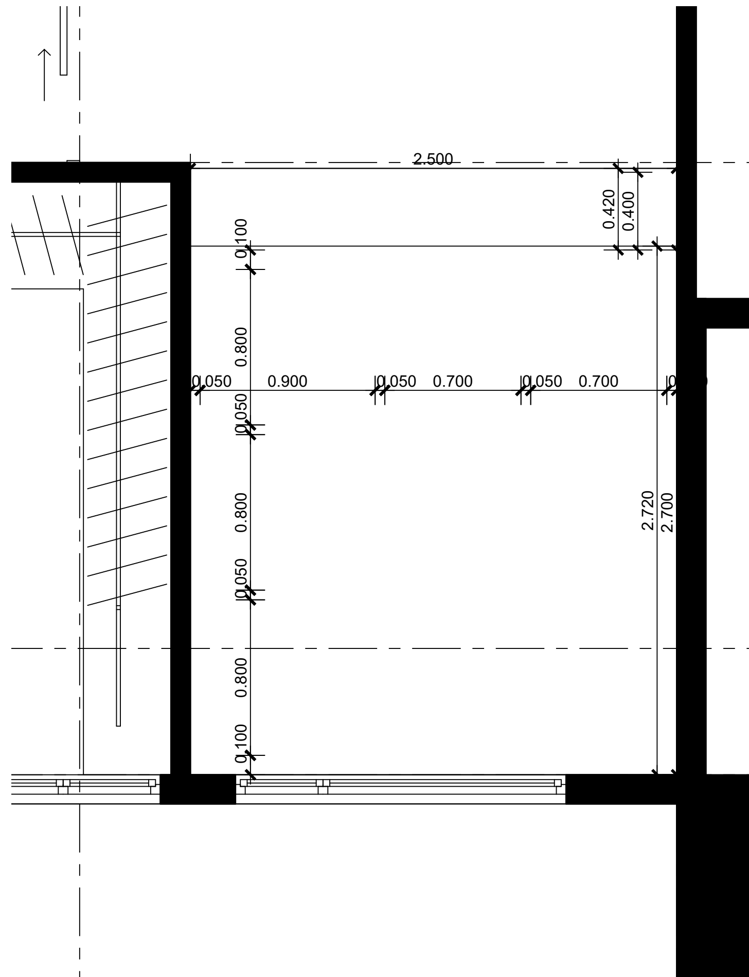
2 TOP WASHITSU 1:20
