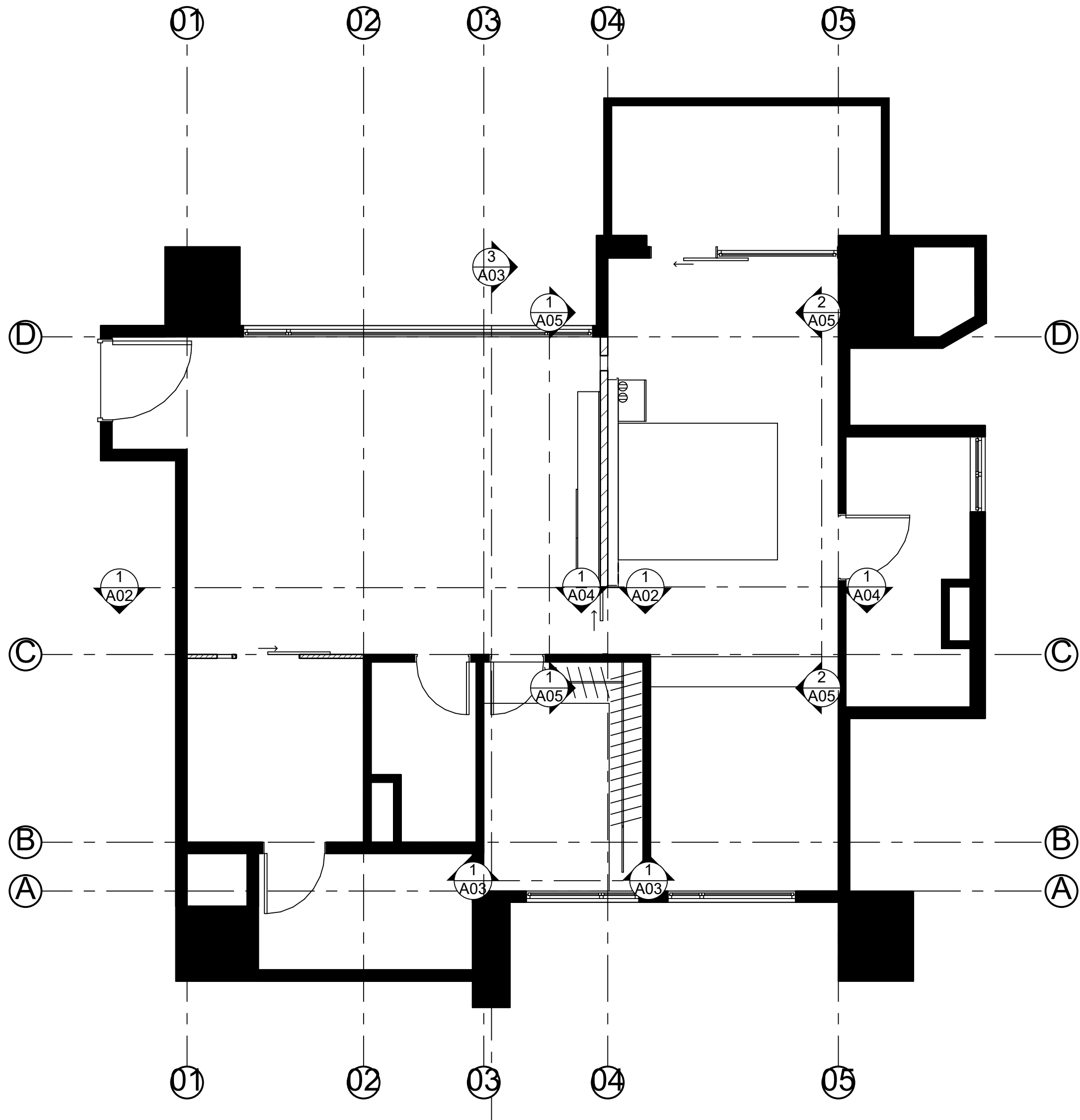
1 FLOOR PLAN 1:50
