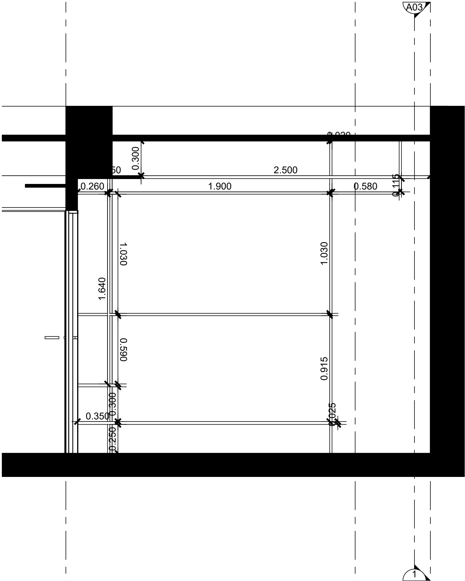
3 WARDROBE SECTION 1:20
